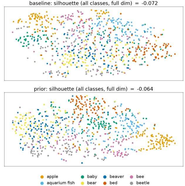
Figure 11: t-SNE of frozen penultimate test features, first eight classes, baseline (top) and prior arm (bottom) at the CIFAR-100 5% cell. The silhouette in each title is computed over all classes in the full feature space, not on the two projected dimensions shown. Reported with its own limitation: the silhouette score over all classes at full dimension moves only from -0.072 to -0.064 , so this projection does not show the +6.3-point feature gap that the linear evaluation measures at this cell. We include it because a reader would otherwise reasonably wonder whether it does.
