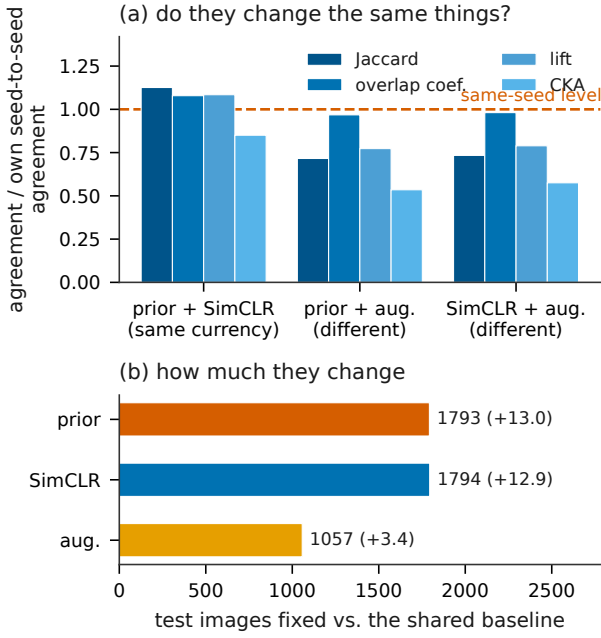
Figure 9: Currency tested directly rather than inferred from magnitudes. All arms are ViT-tiny on CIFAR-100 at 10% with one shared baseline, so the only thing that varies is the fused source. (a) agreement between two interventions in which test images they fix and which representations they learn, each normalized by that intervention’s own seed-to-seed agreement, so 1.0 means the two sources differ no more than two seeds of one of them. Four measures are shown because they do not agree on the size of the effect. (b) the number of images each intervention fixes: the two same-currency sources fix all but one the same number.
