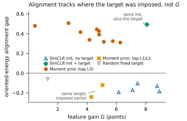
Figure 7: Alignment gap against feature gain, one point per cell, CIFAR-100 / ResNet-18. Filled markers had the moment target during training. The two quantities are independent: every cell whose target was imposed at the tapped stage sits at +0.31 to +0.51 regardless of whether its G is 2.7 or 8.1, and every cell without a target there sits below zero across the same range of G . The two labelled controls are what separate the accounts — the same target imposed two stages earlier leaves no imprint at layer 3, and the same self-supervised initialization as the negative points, with the target added, gives the largest gap measured.
