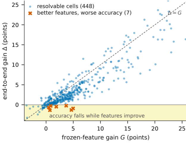
Figure 11: Every resolvable law-scope cell, end-to-end gain against frozen-feature gain. On the dashed diagonal accuracy realizes the feature gain exactly. The shaded quadrant is the patterned failure: features improve measurably while accuracy falls. Only cells whose baseline sits above the crossing are marked, since below it a negative readout is what the account predicts, not a violation of it. Produced by the same audit as Table 7, so the figure and the exception list cannot disagree.
