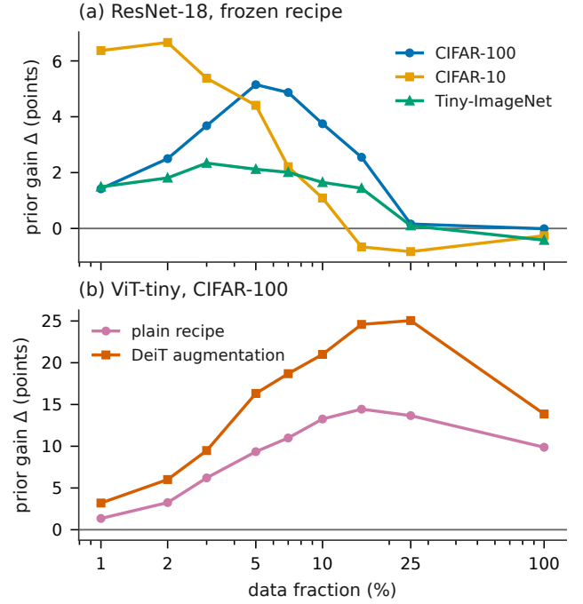
Figure 12: The prior’s gain across the data axis. (a) On convolutional backbones the envelope is unimodal and neutral at sufficiency under the frozen epoch-based recipe; at a matched step budget the right flank does not appear at all (Sec. 3.8). (b) On ViT-tiny the gain is large at every scale, and DeiT-strength augmentation amplifies rather than replaces it.
