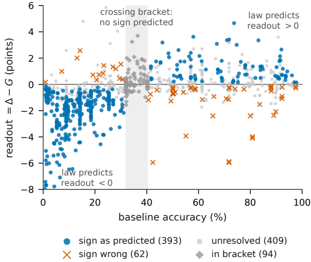
Figure 3: The law, in full: readout = \Delta - G against baseline accuracy for all 958 law-scope cells with \geq 3 seeds on both arms. Shaded band: the measured crossing bracket [31.8, 40.3], inside which no sign is predicted. Only the first two legend entries test the account: of the 455 cells whose readout is resolvable against its own seed-paired uncertainty, 393 fall on the predicted side of zero. The other two entries keep the audit's reach visible: 409 are unresolvable and 94 sit inside the bracket, so the rate is 86.4% at 47.5% coverage against a 75.6% majority-sign baseline. The scatter at fixed baseline is substantial ( R^2 = 0.27 , residual SD 2.0 points): the account predicts the sign of this term, not its value.
