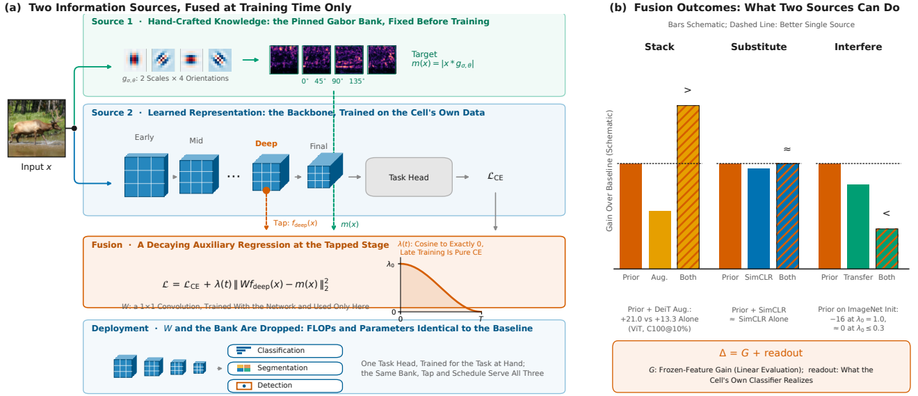
Figure 1: Two information sources, fused at training time only, and the outcomes the benchmark measures. (a) Source 1, hand-crafted knowledge: the pinned Gabor bank turns the input into the fixed oriented-energy target m(x) of Eq. 3 (four of the eight magnitude maps shown), calibrated and fingerprinted before any training and identical for every dataset, backbone and task. Source 2, the learned representation: the same input feeds the unchanged backbone, drawn generically as early, mid, deep and final stages. Fusion: a 1 \times 1 convolution W regresses the tapped deep stage (the third of four in our backbones, f_3 in Eq. 4) onto the target, so training minimizes \mathcal{L} = \mathcal{L}_{CE} + \lambda(t) \|W f_{\text{deep}}(x) - m(x)\|_2^2 , with the cosine schedule (inset) taking \lambda from \lambda_0 to exactly zero, so late training is pure cross-entropy. At deployment W and the bank are dropped, leaving the plain backbone and a task head at FLOPs identical to the baseline; the same bank, tap and schedule serve classification, segmentation and detection, only the head changes. (b) The three outcomes the benchmark measures when two knowledge sources are fused, schematic bars with one measured example each: different currencies can stack, the same currency substitutes, and a strong partner turns the prior into interference (an ImageNet initialization at \lambda_0=1.0 ), which vanishes at \lambda_0 \leq 0.3 . Each cell's gain decomposes as \Delta = G + \text{readout} (Eq. 1), G measured on frozen features under linear evaluation.
