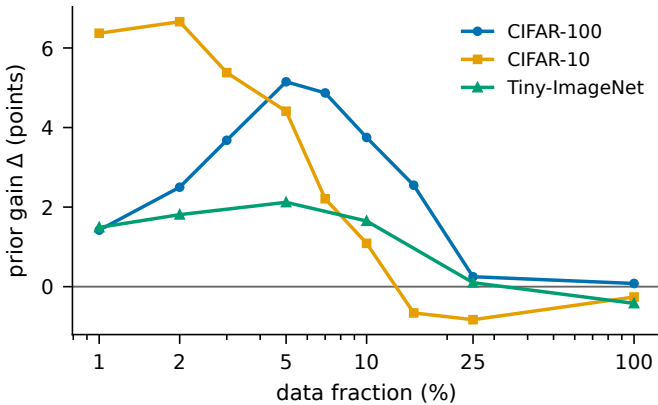
(a) ResNet-18, frozen recipe
