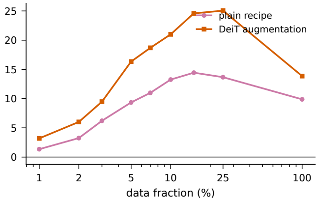
(b) ViT-tiny, CIFAR-100
