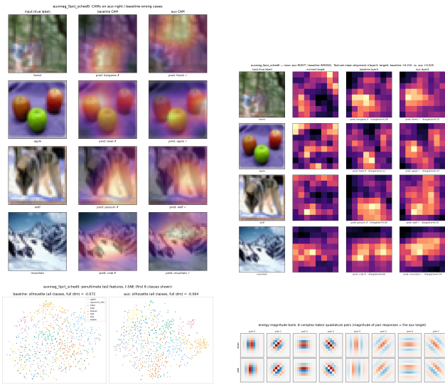
Figure 4: Explainability panels for the CIFAR-100 @5% champion pair. Top: class-activation maps (left) and tapped-stage feature-energy heatmaps (right), baseline vs. prior arm. Bottom left: t-SNE of frozen penultimate features. Bottom right: the pinned 8-pair oriented-energy bank that serves as the auxiliary target.
