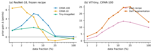
Figure 2: The prior’s gain across the data axis. (a) On convolutional backbones the envelope is unimodal and neutral at sufficiency; the peak tracks task difficulty, not fraction. (b) On ViT-tiny the gain is large at every scale, and DeiT-strength augmentation amplifies rather than replaces it (Section 6).
