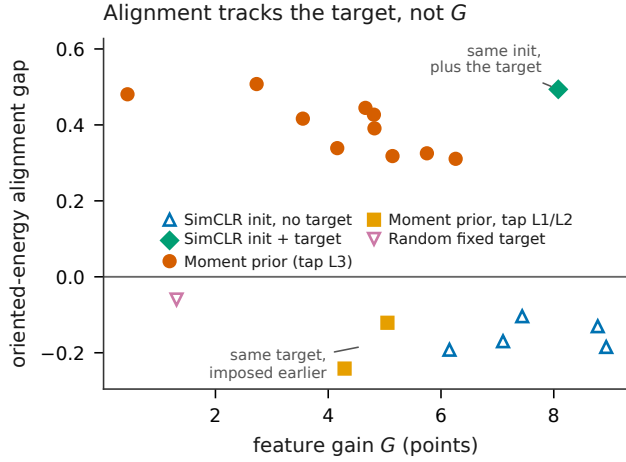
Figure 7: Alignment gap against feature gain, one point per cell, CIFAR-100 / ResNet-18. Filled markers had the moment target during training. The two quantities are independent: every cell whose target was imposed at the tapped stage sits at +0.31 to +0.51 regardless of whether its G is 2.7 or 8.1, and every cell without a target there sits below zero across the same range of G . The two labelled controls are what separate the accounts — the same target imposed two stages earlier leaves no imprint at layer 3, and the same self-supervised initialization as the negative points, with the target added, gives the largest gap measured.
