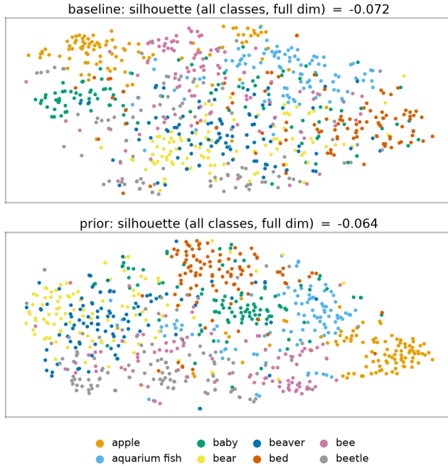
Figure 13: t-SNE of frozen penultimate test features, first eight classes, baseline (top) and prior arm (bottom) at the CIFAR-100 5% cell. The silhouette in each title is computed over all classes in the full feature space, not on the two projected dimensions shown. Reported with its own limitation: the silhouette score over all classes at full dimension moves only from -0.072 to -0.064 , so this projection does not show the +6.3-point feature gap that the linear evaluation measures at this cell. We include it because a reader would otherwise reasonably wonder whether it does.
