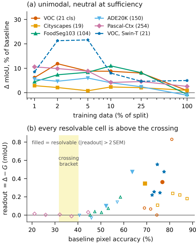
Figure 11: Semantic segmentation, six populations, 200 epochs, three seeds per cell. (a) \Delta as a percentage of each cell's own baseline rather than in absolute mIoU, since the baselines differ eightfold. Read this way the envelopes are unimodal, occupy the same 1–22% band classification does, and go neutral or negative at full data on three populations. (b) Readout against the head's own classification scale (pixel accuracy), not mIoU: the crossing bracket is an accuracy bracket, and scoring the law on mIoU puts every dense cell on the wrong flank. Filled markers are the resolvable cells; all sit above the bracket, so segmentation confirms the law's positive branch and cannot test its negative one.
