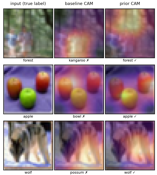
Figure 6: Where the class evidence sits, CIFAR-100 at 5%. The three rows are selected cases (prior arm correct, baseline wrong), so they show what the difference looks like where it is present, not how often. The evidential quantity is measured over the whole test set instead: the Gini coefficient of each class-activation map normalized to sum one — higher means evidence concentrated at fewer locations — gives 0.253 for the baseline against 0.273 for the prior arm over 2,000 images ( 8.6\sigma ), both arms scored on the same images. The prior’s evidence is measurably more concentrated, by a modest amount — not the categorical difference the three rows suggest.
