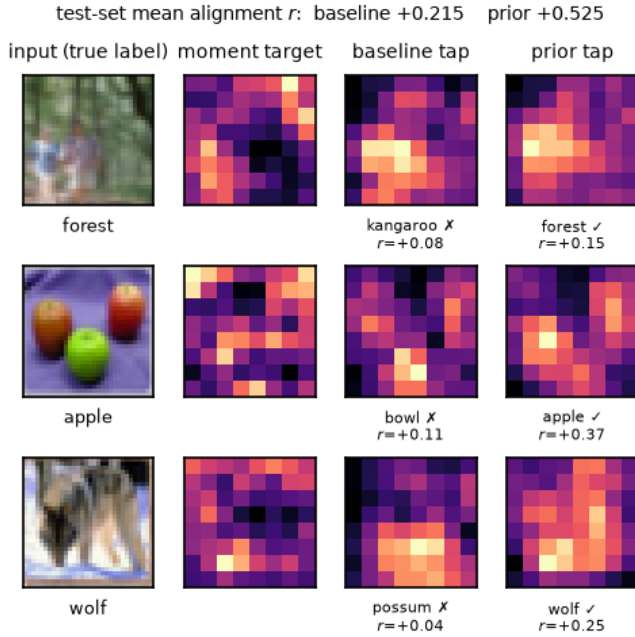
Figure 5: The spectral imprint at the tap, CIFAR-100 at 5%. Columns: input, the fixed moment target, and the tapped-stage energy of the baseline and prior arms. Over the whole test set the alignment between tapped features and the target is +0.215 for the baseline and +0.525 for the prior arm; the per-row values are printed beneath each map. The three rows are selected cases where the prior arm predicts correctly and the baseline does not, so they illustrate the alignment difference rather than sample it, and only the test-set-wide figure should be read as evidence.
