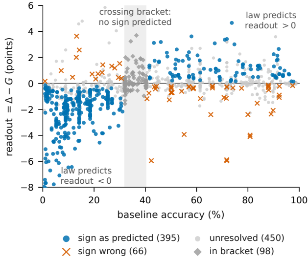
Figure 4: The law, in full: \text{readout} = \Delta - G against baseline accuracy for all 1,009 law-scope cells with \geq 3 seeds on both arms. Shaded band: the measured crossing bracket [31.8, 40.3], inside which no sign is predicted. Only the first two legend entries test the account: of the 461 cells whose readout is resolvable against its own seed-paired uncertainty, 395 fall on the predicted side of zero. The other two are shown because omitting them would misrepresent how much of the grid the audit can speak to. The scatter at fixed baseline is substantial ( R^2 = 0.26 , residual SD 2.0 points): the account predicts the sign of this term, not its value.
