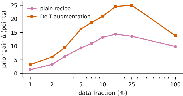
(b) ViT-tiny, CIFAR-100
