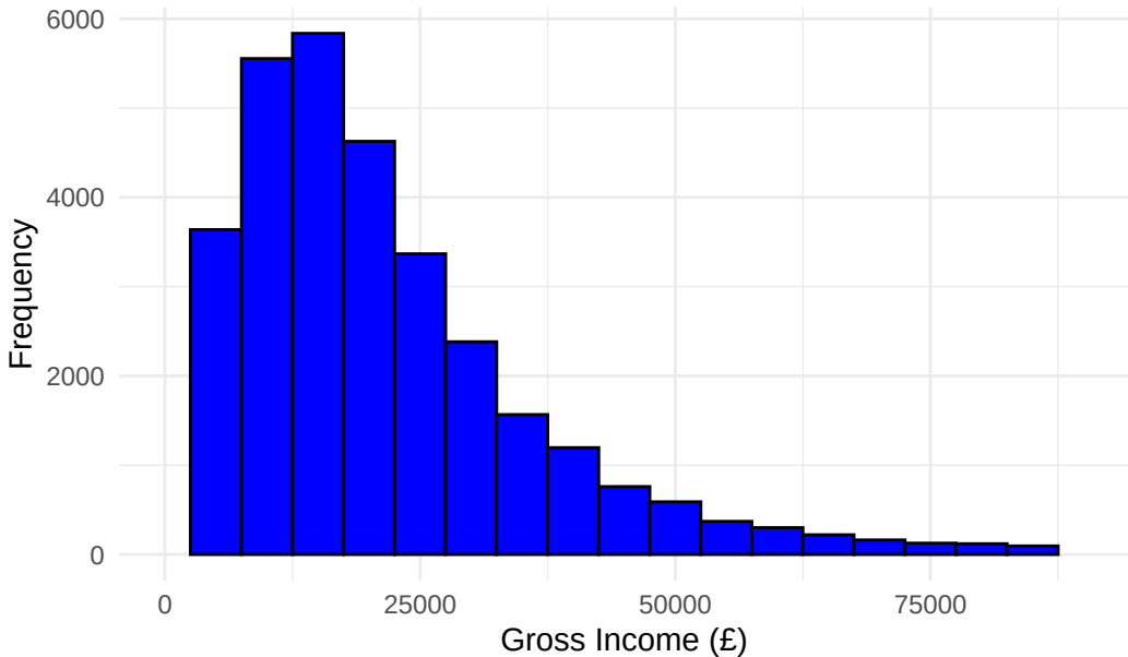
Distribution of Gross Household Income
