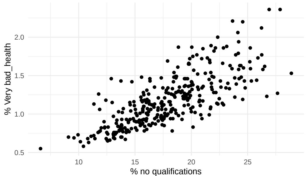
Scatterplot of % people in Very bad health vs & % people No Q
