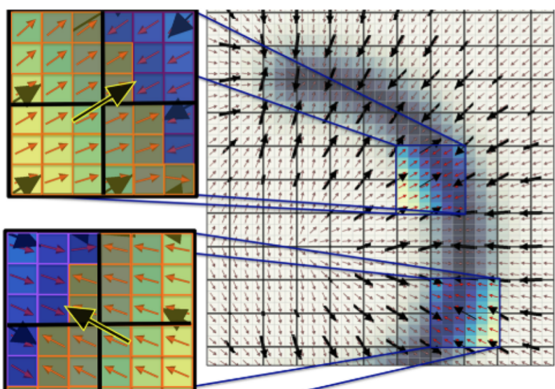
(b) DFG partitioning at a curved fracture
