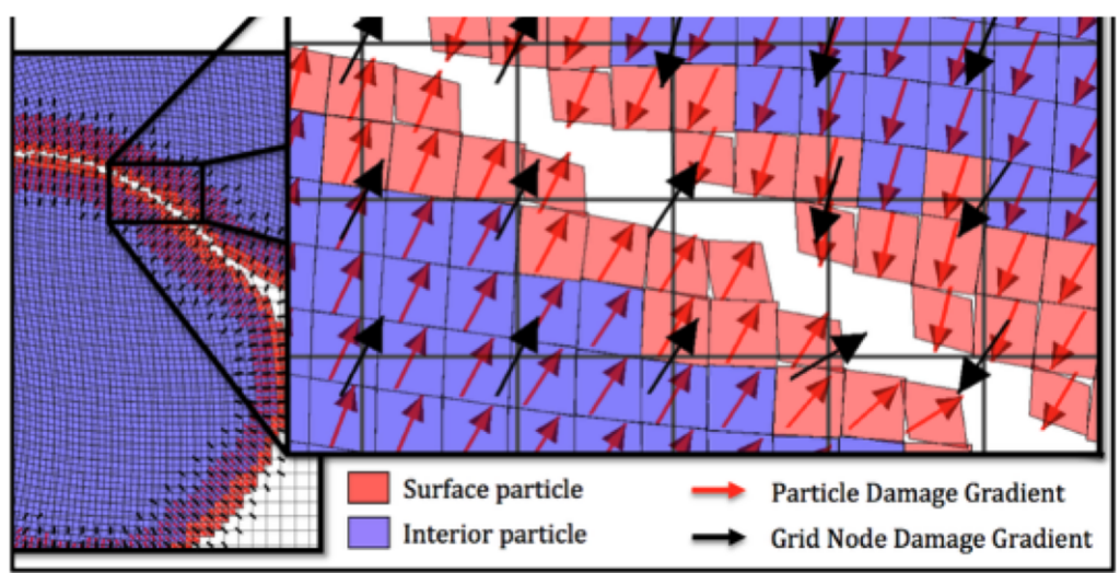
(c) DFG with painted surface flags
