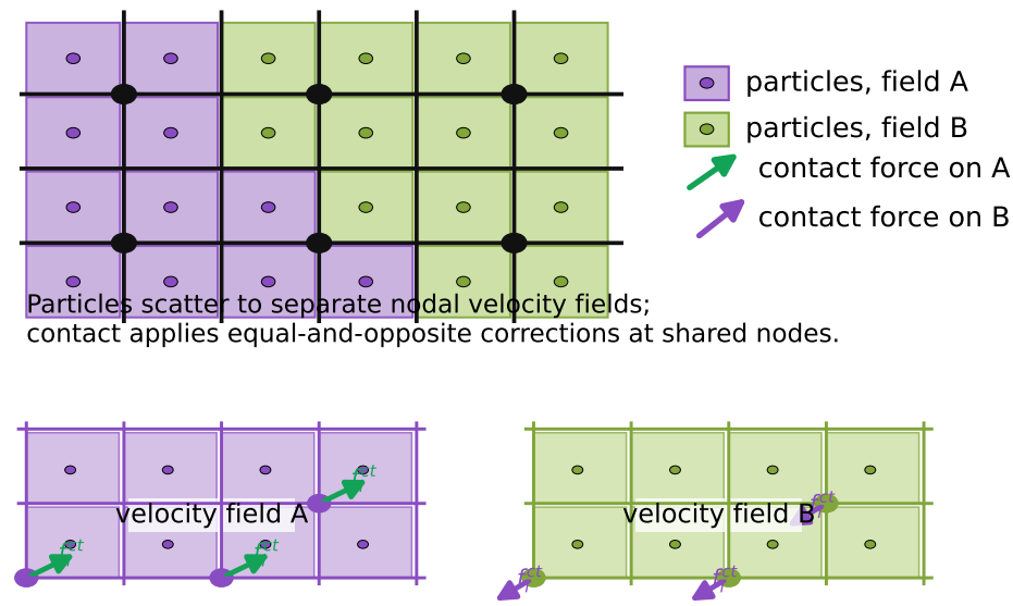
(a) Prescribed multi-field contact
