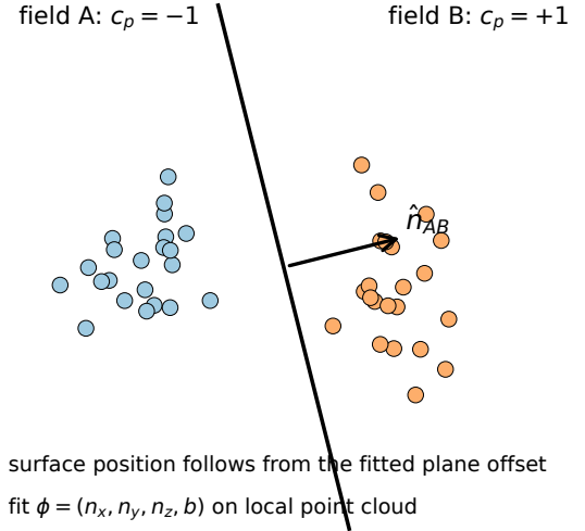
Logistic-regression plane
