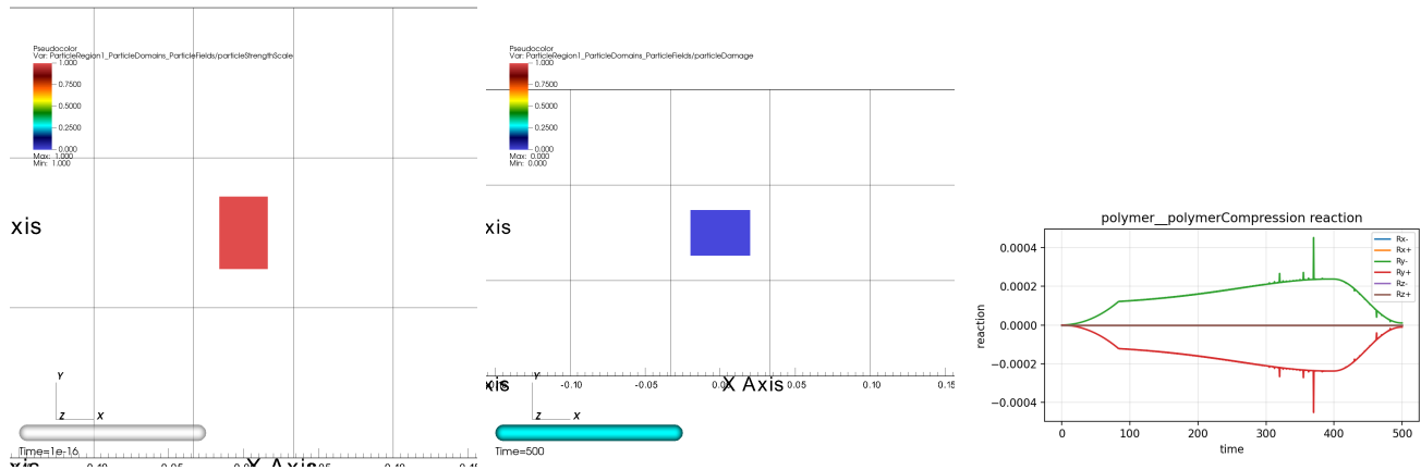
Figure 23: Initial state, final state, and history/comparison plot for polymer__polymerCompression.
