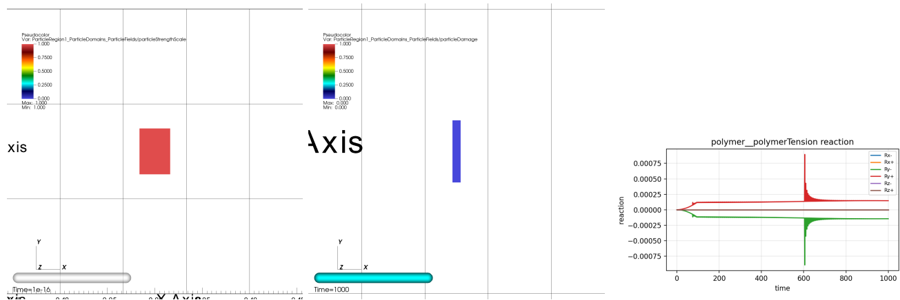
Figure 26: Initial state, final state, and history/comparison plot for polymer__polymerTension.
