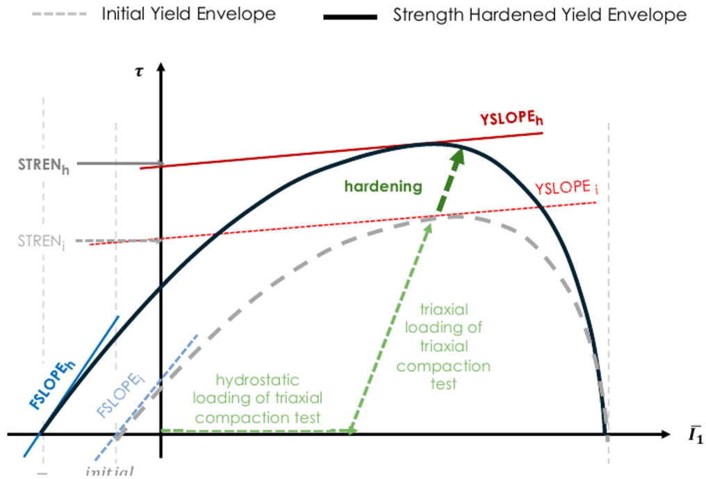
Figure 2.4: Geomechanics formulation diagrams adapted from Malenda, Homel, Kibikas, Choens, Shalev, and Lyakhovsky [47]. (a) The shear-limit function is multiplied by a cap function to obtain a pressure-sensitive strength surface. (b) Creep first relaxes the beginning-of-step state, then an elastic trial stress is computed, and a plastic return is performed to the evolved surface. (c) Strain hardening expands the strength envelope and shifts the triaxial-loading response.
