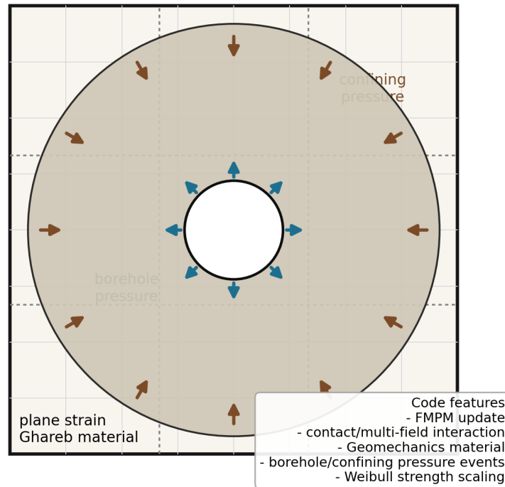
Figure 13: Schematic for borehole_Ghareb.
