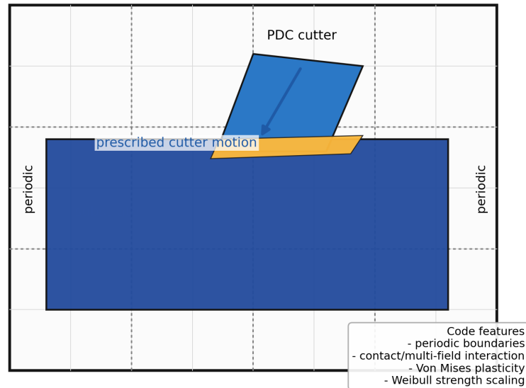
Figure 19: Schematic for pdc.
