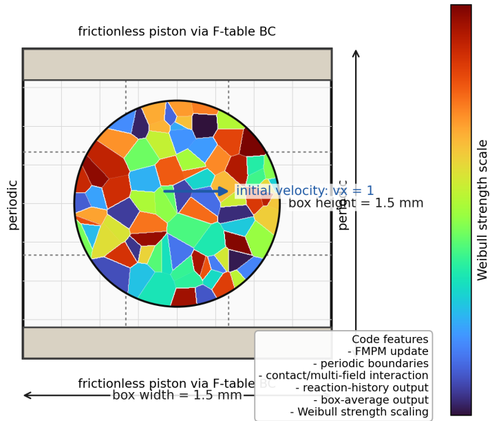
Figure 1: Schematic for brazilianDisk_FMPM.
