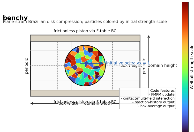
Figure 11: Schematic for benchy.
