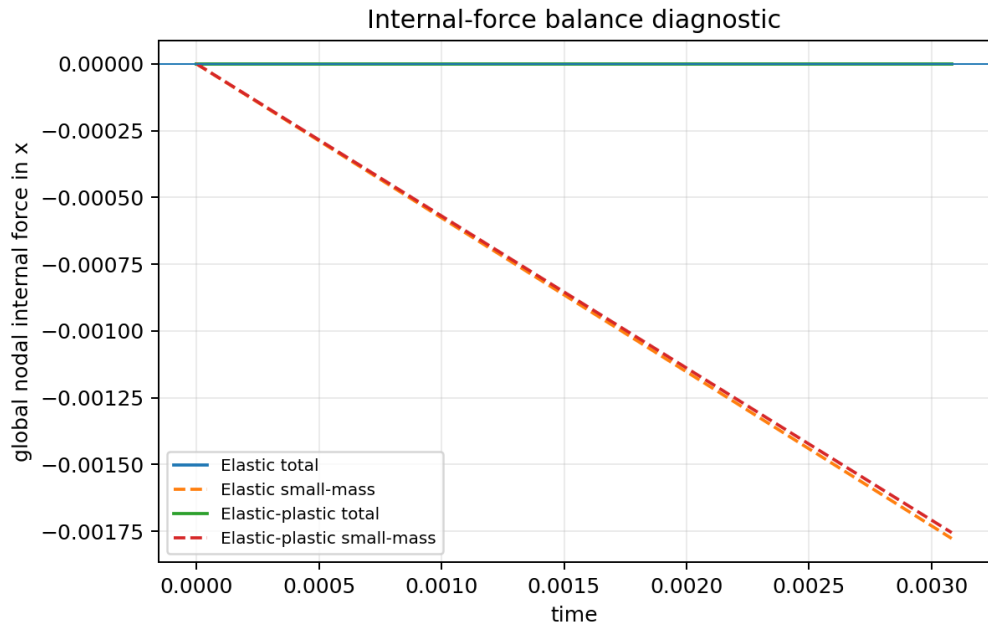
Figure 3: Global x-component of the nodal internal-force balance, including the contribution carried by small-mass nodes.
