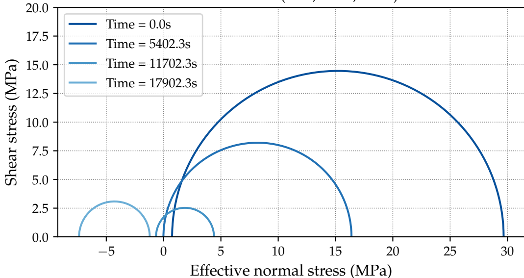
Stress state at (0.10, -0.00, -0.03)
