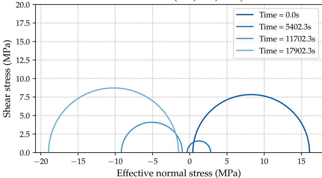
Stress state at (0.00, 0.10, -0.03)
