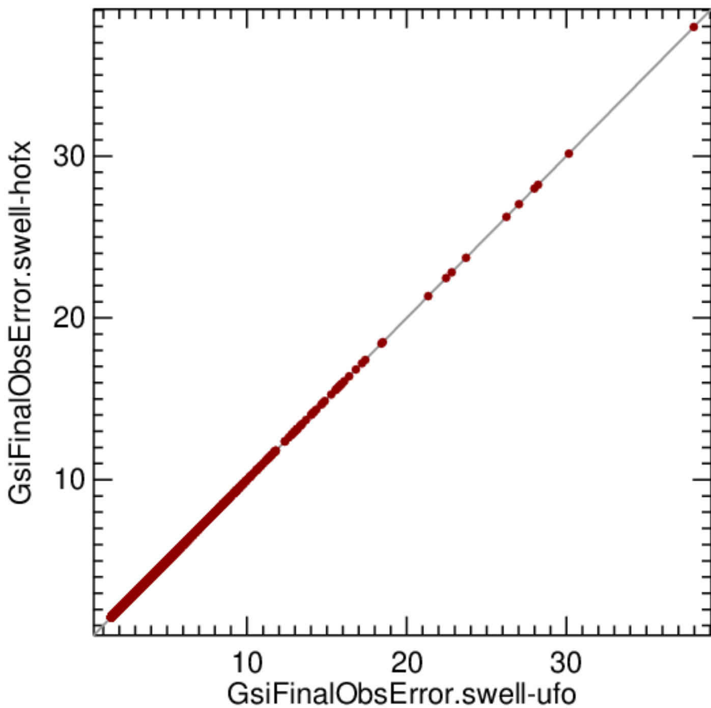
sonde windNorthward
