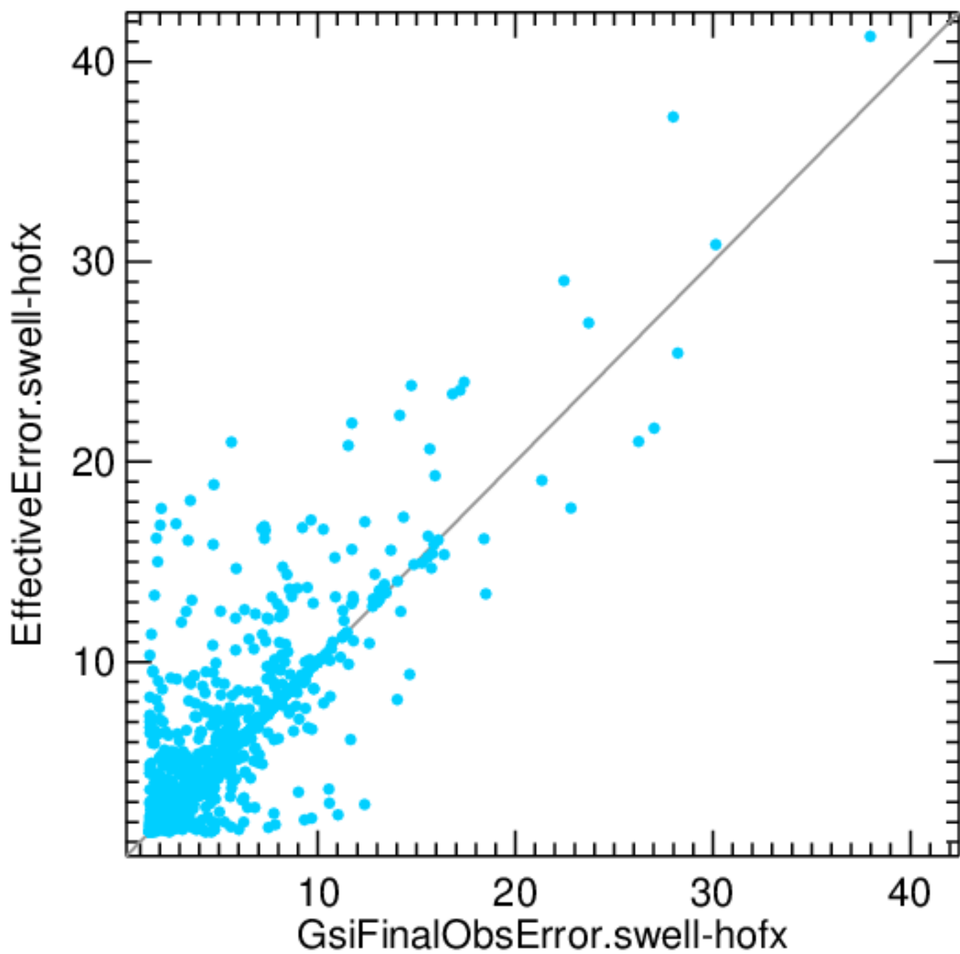
sonde windNorthward
