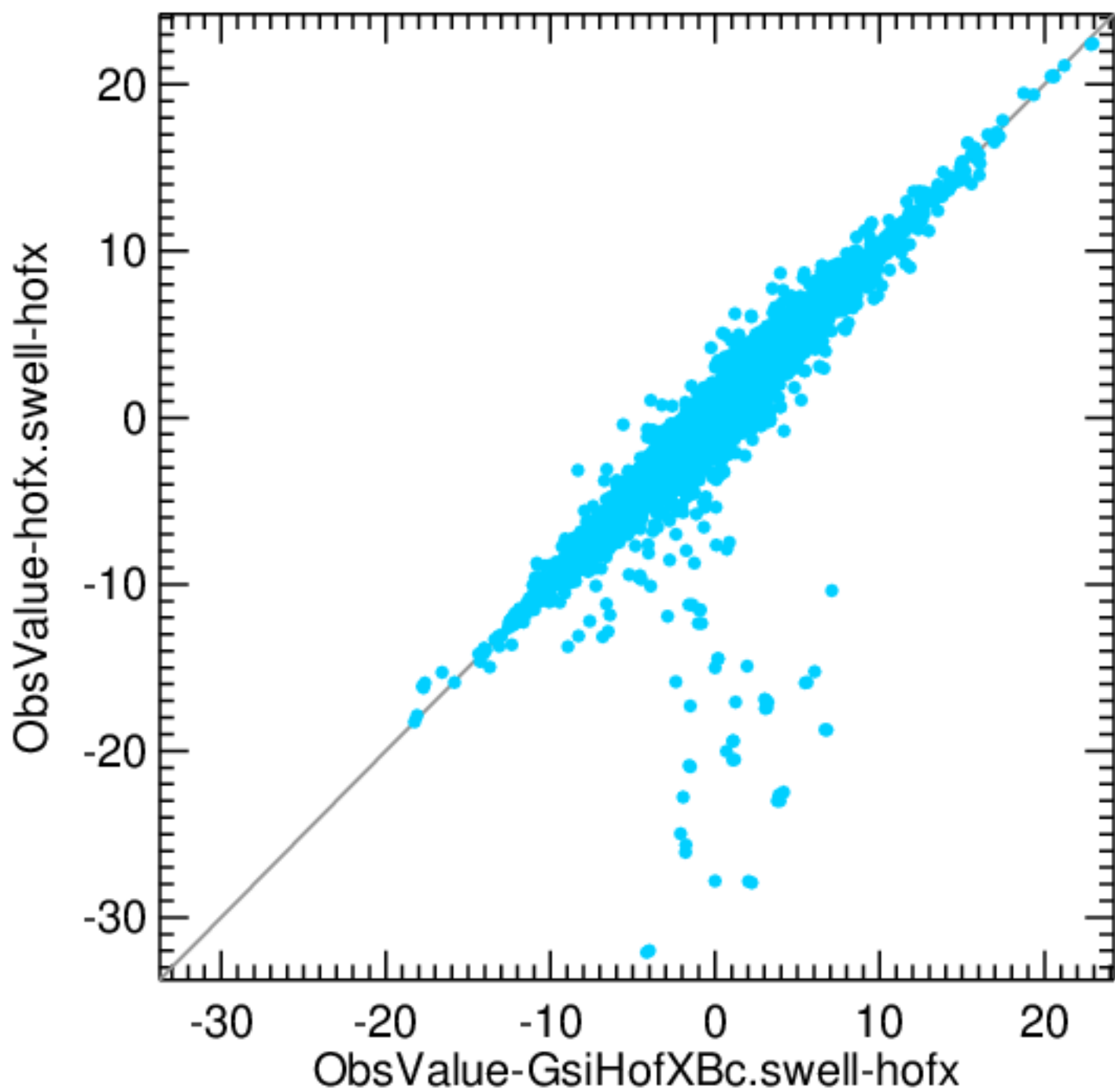
sonde windNorthward
