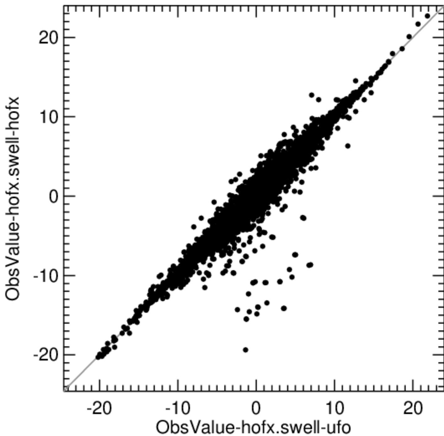
sonde windEastward
