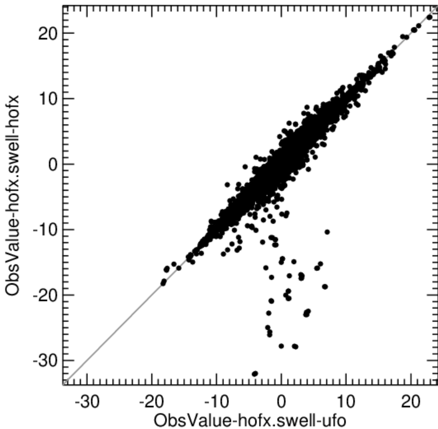
sonde windNorthward
