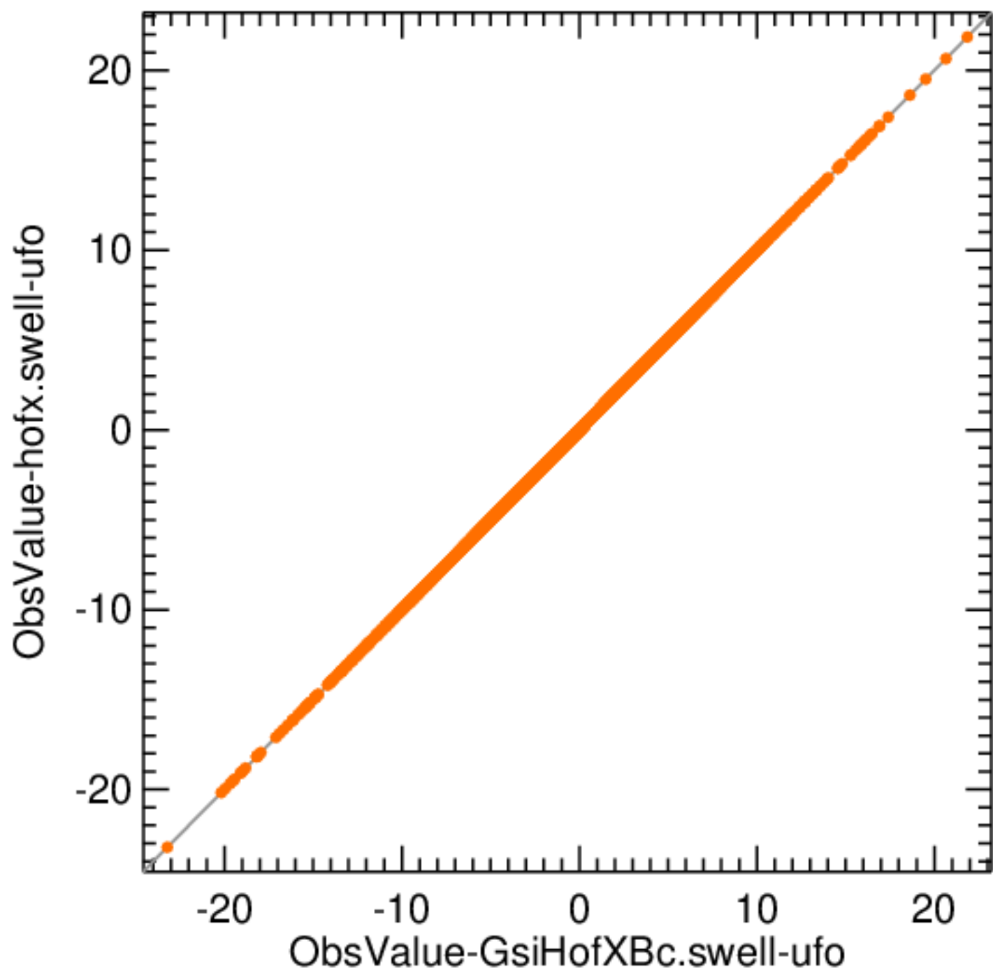
sonde windEastward
