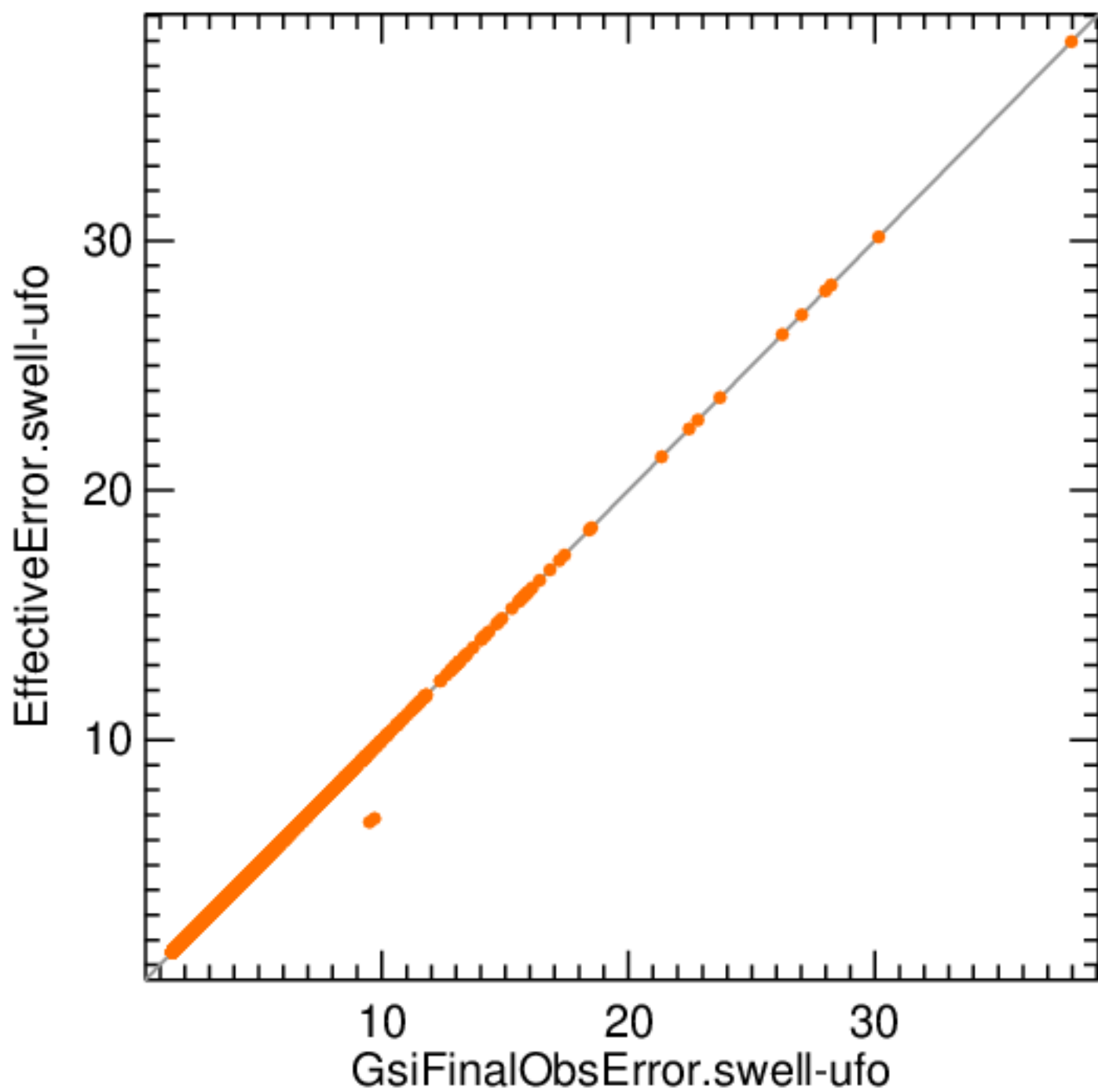
sonde windEastward
