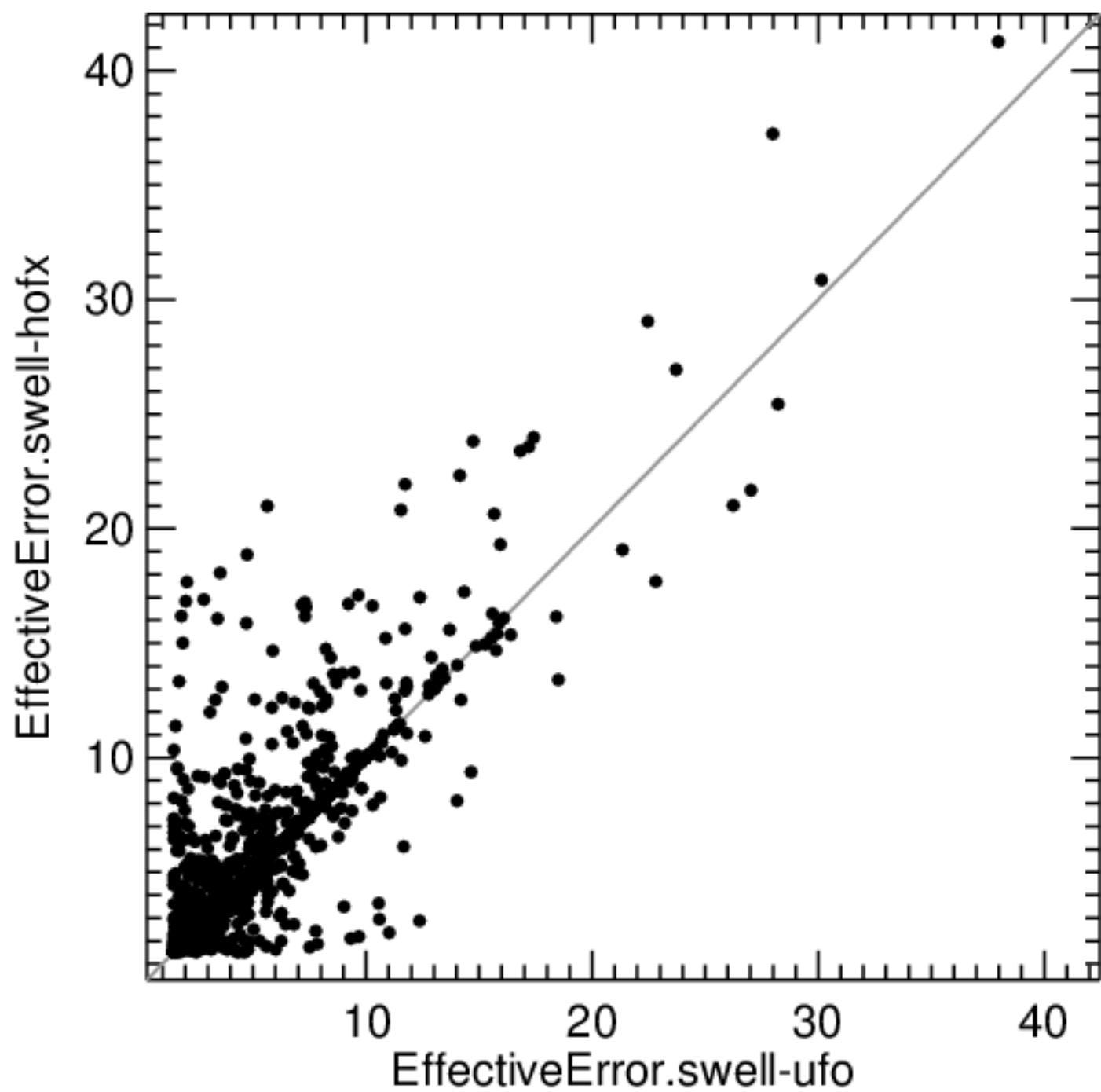
sonde windNorthward
