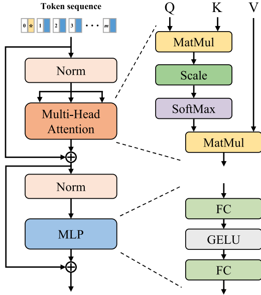
Fig. 4. The structure of the Transformer encoder, where FC is a fully connected layer and \oplus is element-wise addition. [\ast] is the classification token.
