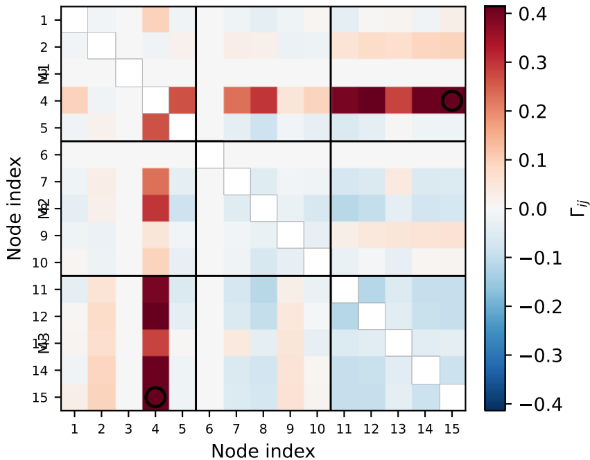
Pairwise synergy in a Modular multistable BN
