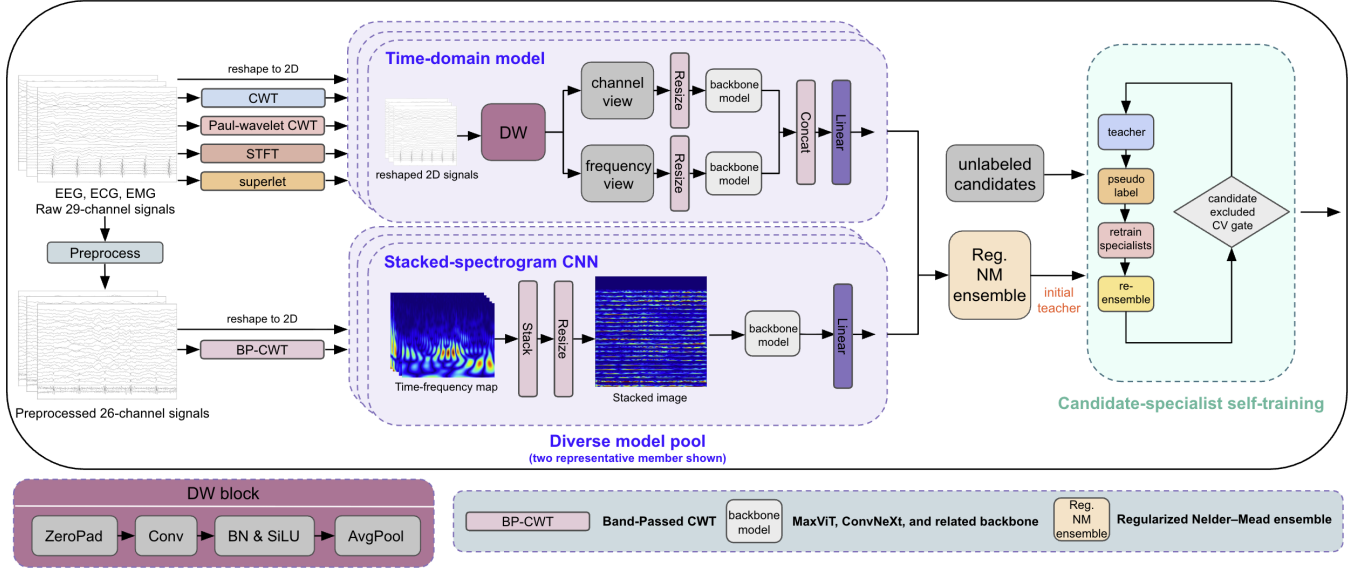
Figure 1: System data-flow. An inductive pipeline—preprocessing, five time–frequency representations, a diverse model pool (two representative members shown), and a regularized Nelder–Mead ensemble—is broken past saturation by candidate-specialist transductive self-training, whose teacher iteration is gated by candidate-excluded cross-validation. Backbones are shown as boxes, not internal architectures: the spectrogram members use off-the-shelf timm backbones [30, 37], while the multi-view model is our simplified re-implementation of a public design [25].
