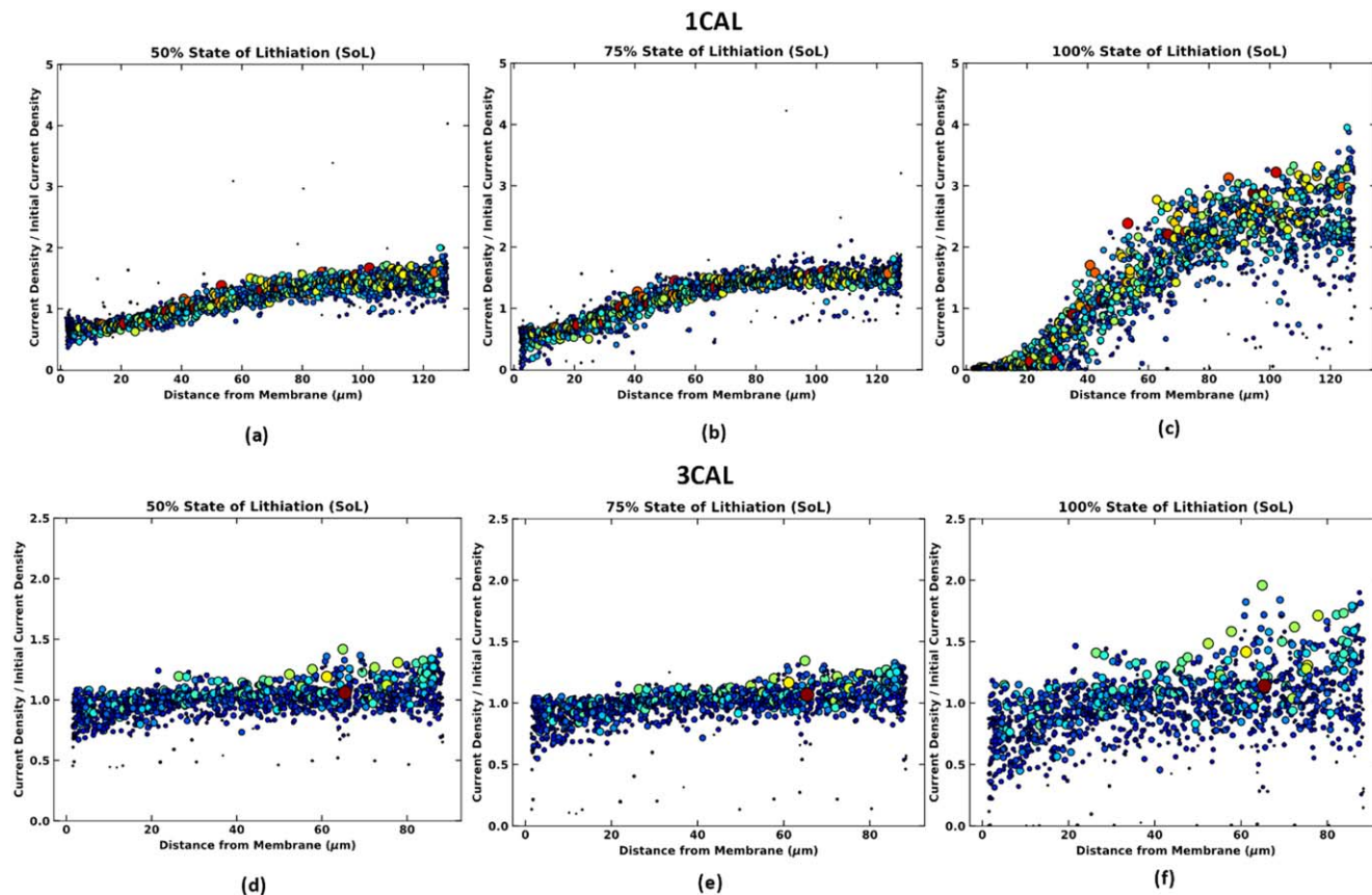
Figure 8. (a)–(c) Deviation of current density from initial current density at 50, 75 & 100% SoL respectively for 1CAL cathode, (d)–(f) Deviation of current density from initial current density at 50, 75 & 100% SoL respectively for 3CAL cathode. The color of circles indicates the size of active material particles with red and blue referring to big and small particles respectively.
