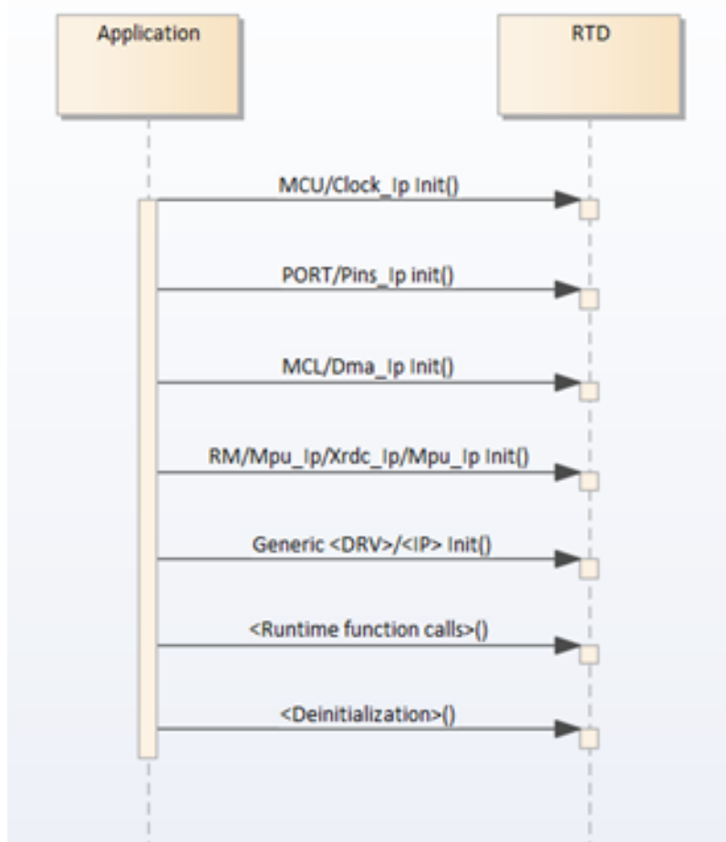
Figure 5.2 Non-AUTOSAR Sequence diagram
