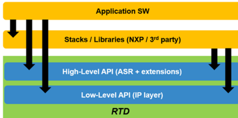
Figure 5.1 RTD Usage in non-ASR Context
