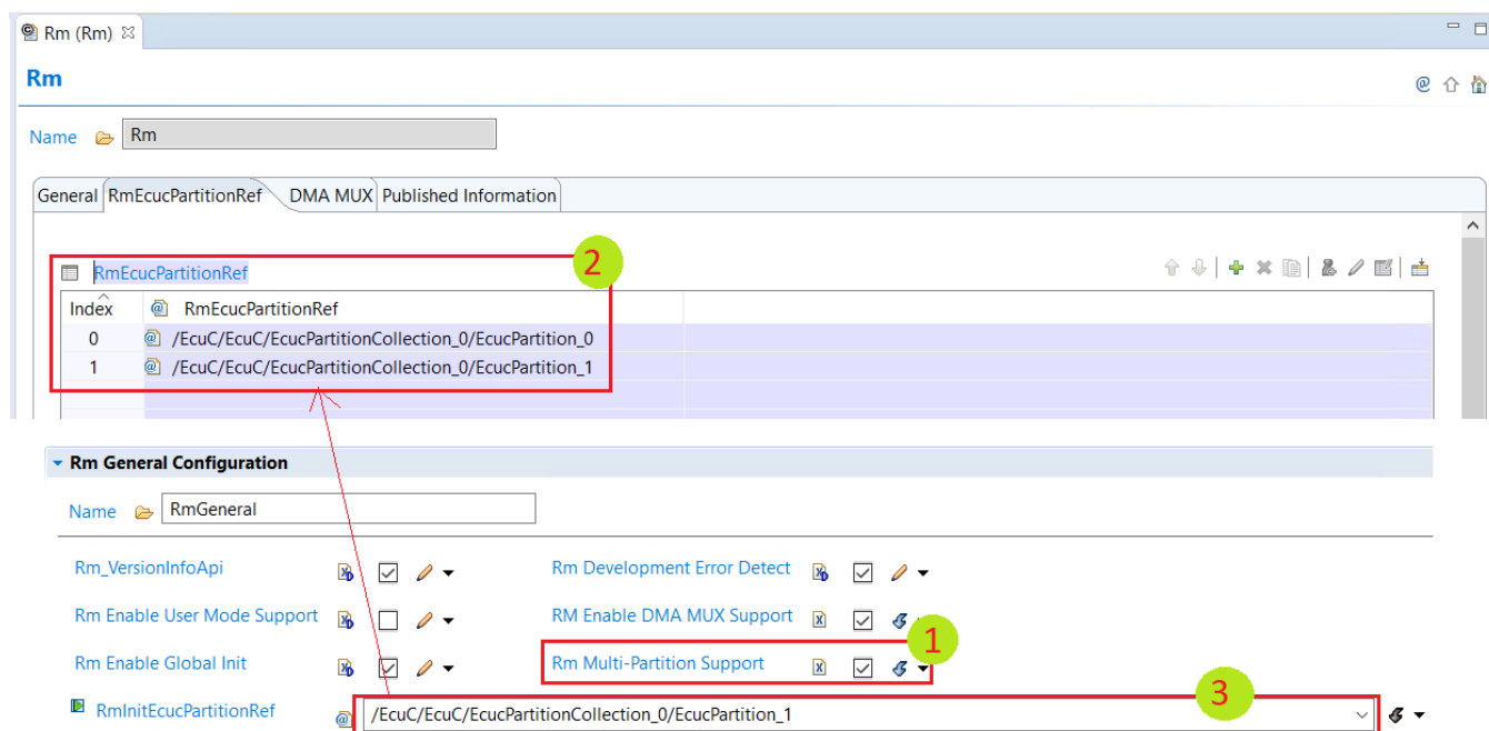
Figure 5.1 Multi-partition configuration
