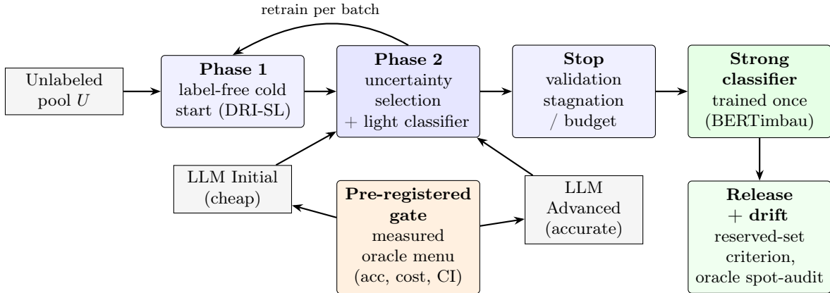
Figure 1: FALCO architecture. A label-free cold start (Phase 1) seeds an uncertainty loop with a cheap classifier (Phase 2); a pre-registered gate assigns measured LLM oracles to phases by budget/quality; the loop stops by validation stagnation; the strong classifier is trained once on the collected set; release and drift monitoring reuse the cheap oracle as an audit instrument.
