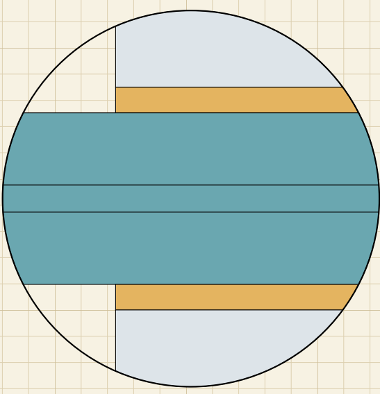
REPRESENTATIVE CRUSH SEAL / ENLARGED
