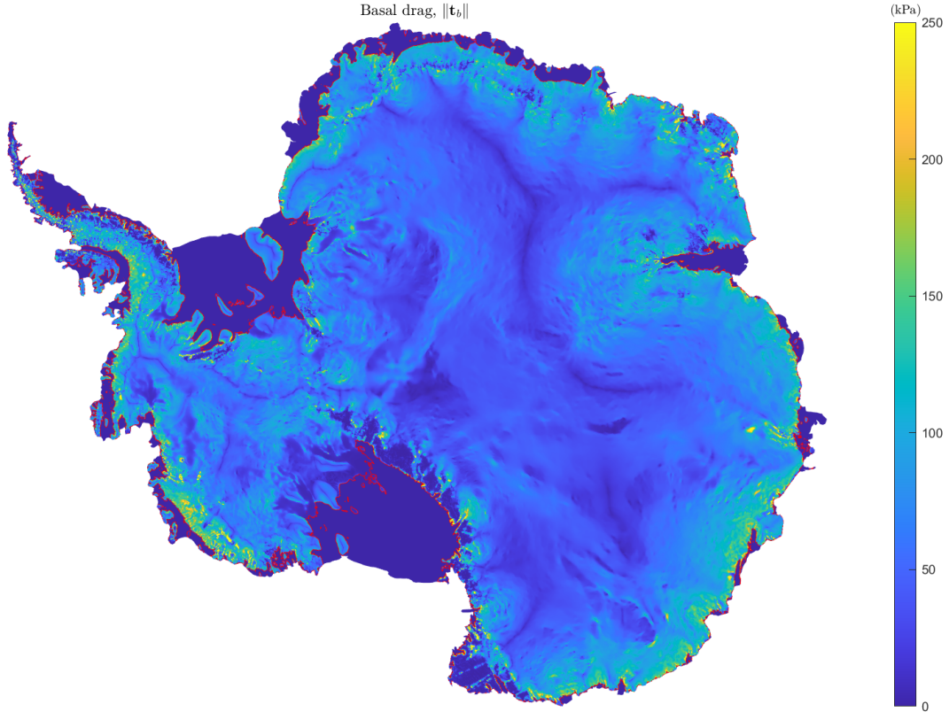
Figure 6.9: Modelled basal drag for Cornford sliding law given by Eq. (1.164) for m = 3 and \mu = 1/2 , and perfect hydrological connection, Eq. (1.187), using the A and C distributions shown in Figs. 6.6 and 6.7.
