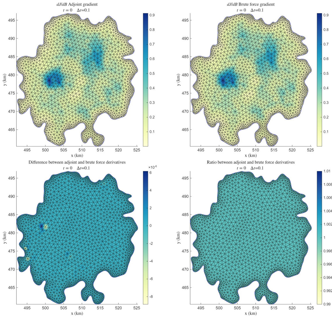
Figure 6.13: Gradient calculation, dJ/dB , done with adjoint and finite differences. This test was done for the Hoffsjökull ice cap in Iceland.
