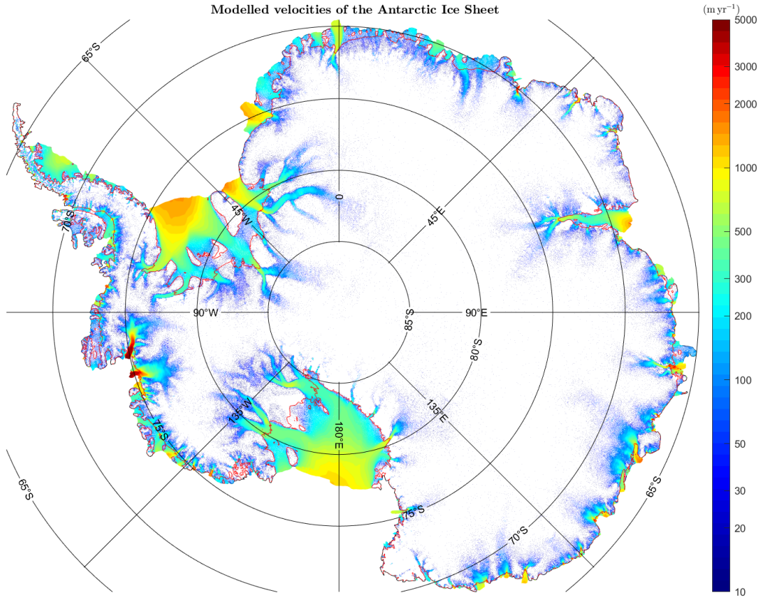
Figure 6.8: Modelled velocities for the A and C distributions in Figs. 6.6 and 6.7.
