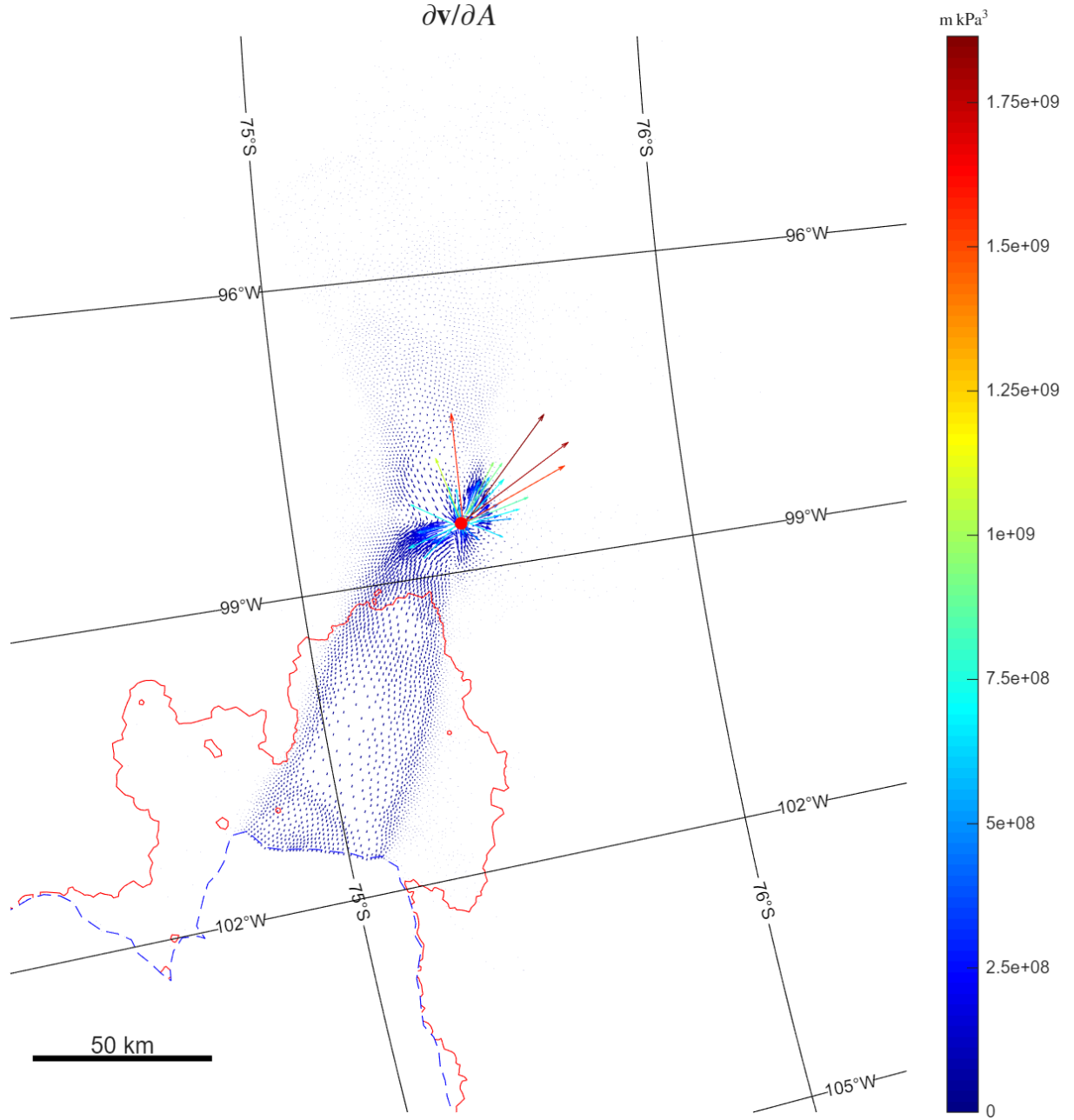
Figure 6.1: Sensivities of velocities to changes in A at one node. The full sensitivity matrix \xi was calculated solving Eq. (6.8), providing the sensitivity of all nodal velocities to any nodal A values. The FE mesh had 31,717 nodes and calculating the sensitivities took about 3 min. The examples is for Pine Island Glacier, West Antarctica.
