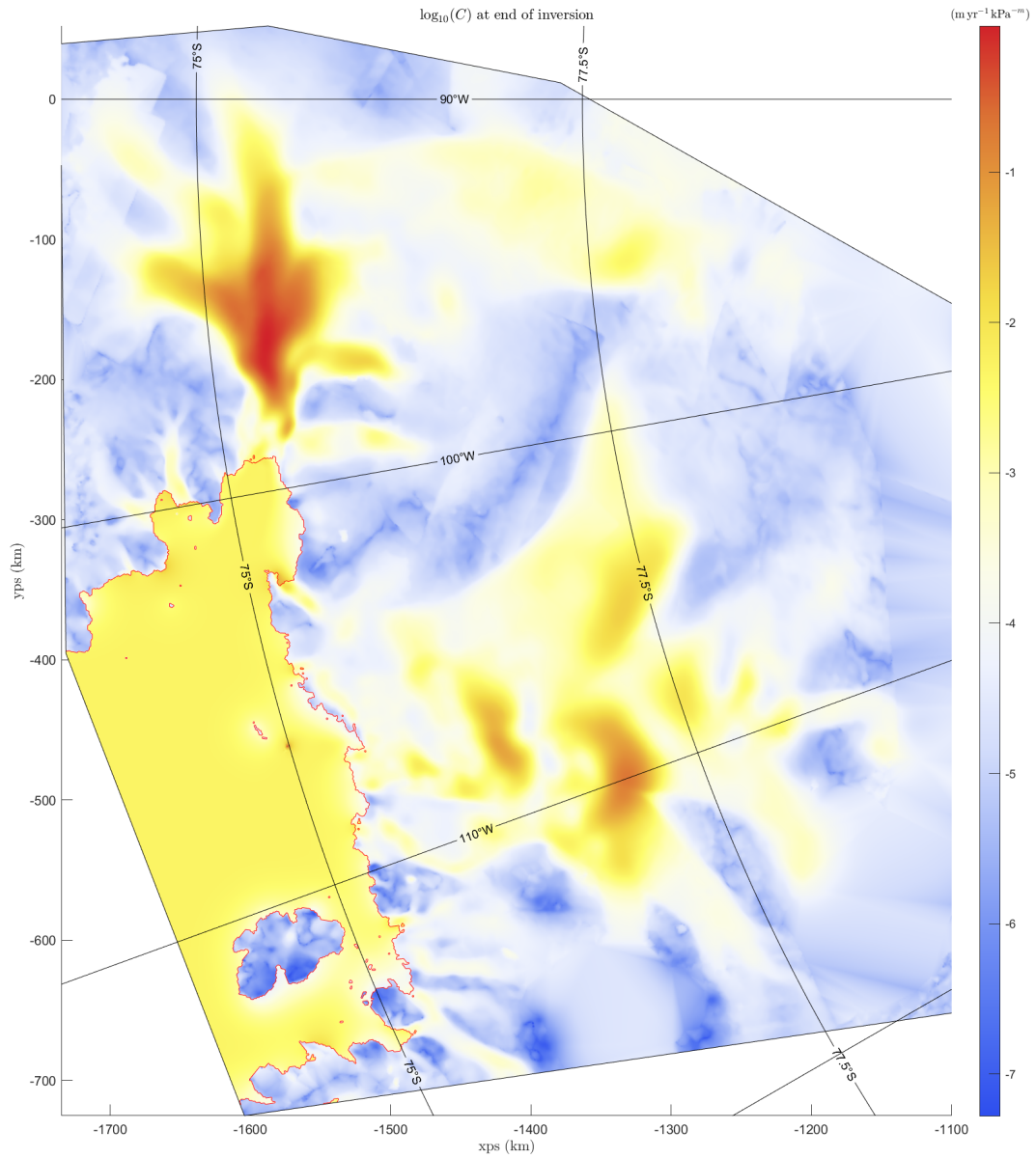
Figure 6.5: Example of an estimated C distribution over a section of West Antarctica using the Cornford sliding law with the stress exponent m = 3 and the coefficient of kinetic friction \mu_k = 1/2 . Here \gamma_a = 1 and \gamma_s = 100,000 .
