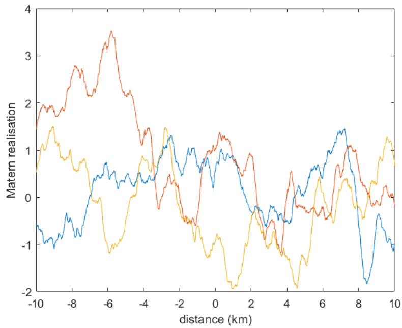
Figure 6.11: Three examples of Matérn realisations for \rho = 3 km, \nu = 1 , d=2 and \sigma = 1 .
