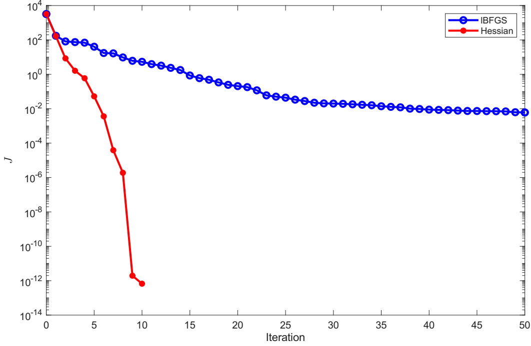
Figure 6.3: Comparison between an inversion using the Hessian and the IBFGS methods. The function J is the cost function. This example was done for a relatively small problem where calculating the full Hessian using brute-force was feasible, using finite-differences of the gradient as shown in Eq. (6.29).
