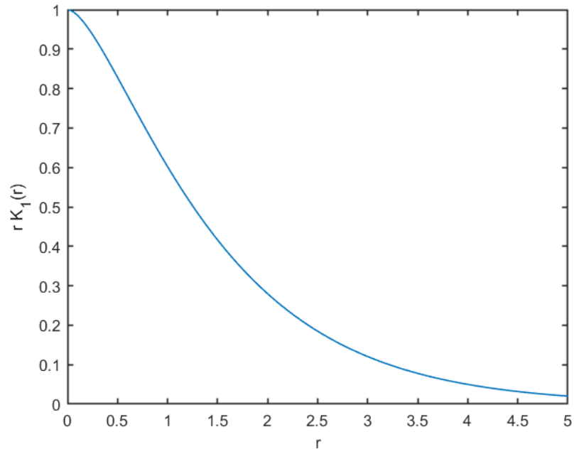
Figure 6.10: The function rK_1(r) appearing in Eq. (6.43)
