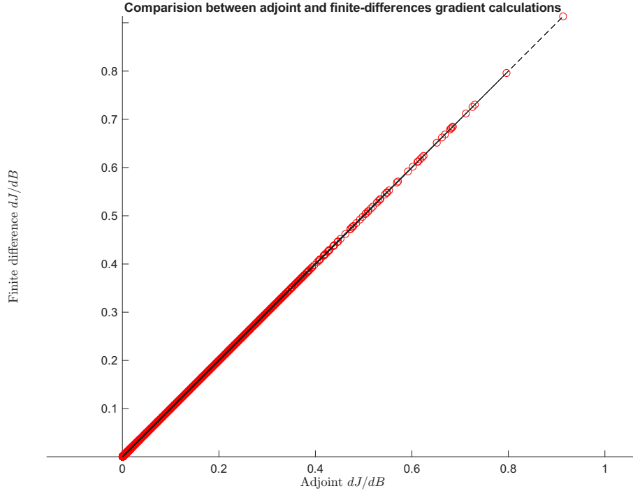
Figure 6.15: Comparison between adjoint and finite differences gradient calculations. This test was done for the Hoffsjökull ice cap in Iceland.
