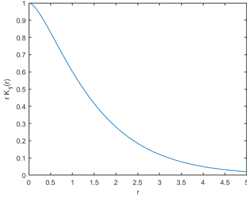
Figure 6.13: The function rK_1(r) appearing in Eq. (6.52)
