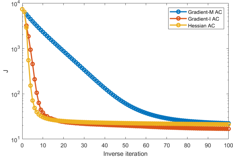
Figure 6.15: An example showing cost function reduction as a function of inverse iterations, when inverting for both A and C using a gradient based approach with l^2 and L^2 gradients, labelled with I and M respectively, and using a Hessian-based inversion where the Hessians of the regularisation terms are exact, and the Hessian of the A and C terms of the misfit are approximated using the fixed-point approach. See section 6.10, for discussion of the l^2 and L^2 gradients.
