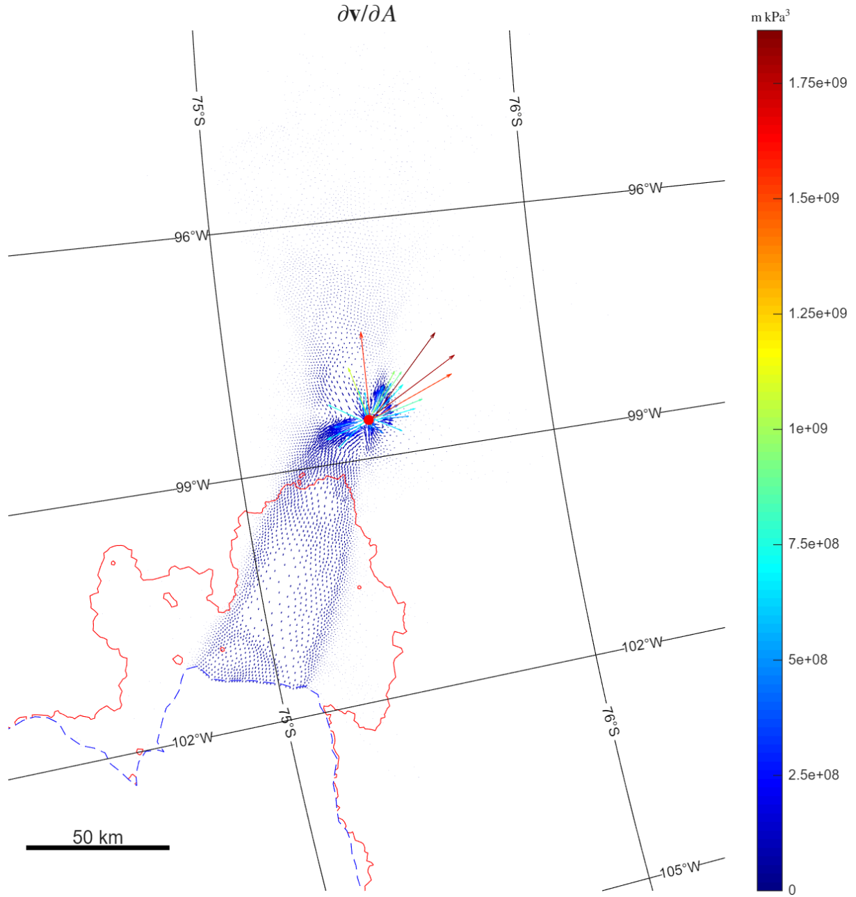
Figure 6.1: Sensivities of velocities to changes in A at one node. The full sensitivity matrix \xi was calculated solving Eq. (6.10), providing the sensitivity of all nodal velocities to any nodal A values. The FE mesh had 31,717 nodes and calculating the sensitivities took about 3 min. The examples is for Pine Island Glacier, West Antarctica.
