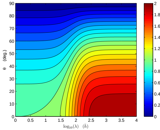
Figure 18.3: The phase speed ( \|v_p\| ) of the full-system solution as a function of wavelength \lambda and orientation \theta of the sinusoidal perturbations with respect to mean flow direction. The mean surface slope is \alpha=0.002 and the slip ratio is \bar{C}=100 , and n=m=1 . The plot has been normalised with the non-dimensional surface velocity \bar{u}=\bar{C}+1=101 of the full-system solution.
