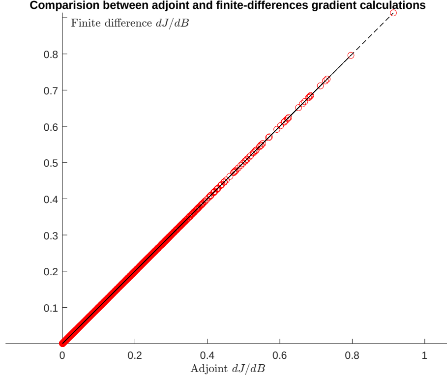
Figure 6.18: Comparison between adjoint and finite differences gradient calculations. This test was done for the Hoffsjökull ice cap in Iceland.
