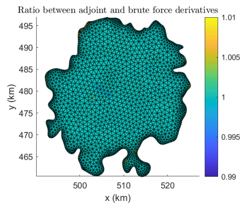
Figure 6.15: Gradient calculation, dJ/dC , done with adjoint and finite differences. This test was done for the Hoffsjökull ice cap in Iceland.
