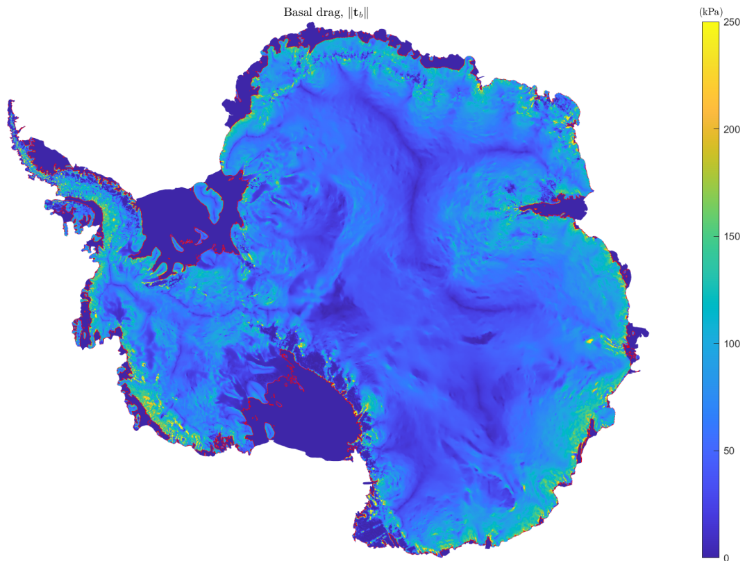
Figure 6.10: Modelled basal drag for Cornford sliding law given by Eq. (1.163) for m = 3 and \mu = 1/2 , and perfect hydrological connection, Eq. (1.186), using the A and C distributions shown in Figs. 6.7 and 6.8.
