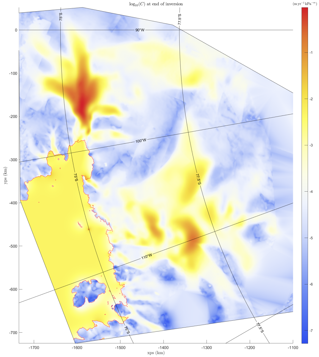
Figure 6.6: Example of an estimated C distribution over a section of West Antarctica using the Cornford sliding law with the stress exponent m = 3 and the coefficient of kinetic friction \mu_k = 1/2 . Here \gamma_a = 1 and \gamma_s = 100,000 .
