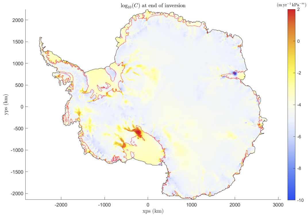
Figure 6.8: Example of an estimated basal slipperiness ( C ) distribution for Antarctica for Weertman sliding law where m = 3 . Here \gamma_a = 1 and \gamma_s = 10,000 .
