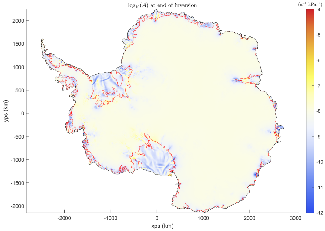
Figure 6.7: Example of an estimated A distribution for Antarctica for n = 3 . Here \gamma_a = 1 and \gamma_s = 100,000 .
