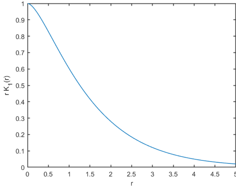
Figure 6.11: The function rK_1(r) appearing in Eq. (6.52)
