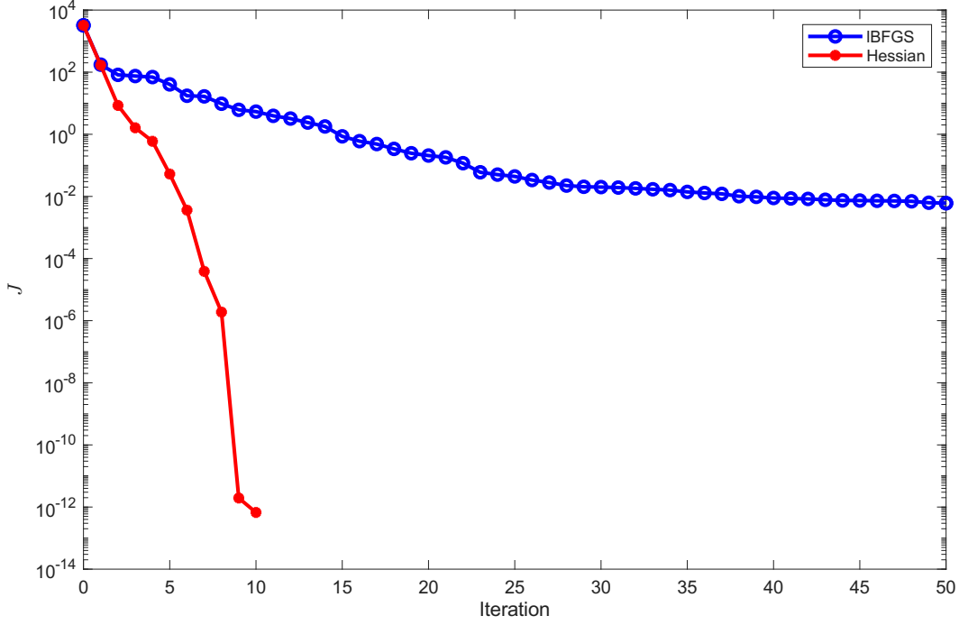
Figure 6.4: Comparison between an inversion using the Hessian and the LBFGS methods. The function J is the cost function. This example was done for a relatively small problem where calculating the full Hessian using brute-force was feasible, using finite-differences of the gradient as shown in Eq. (6.38).
