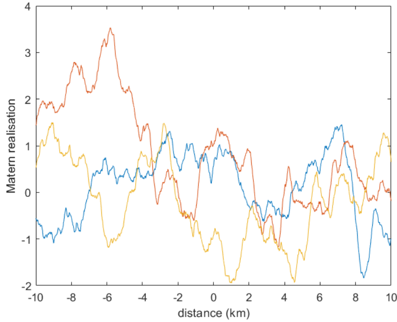
Figure 6.12: Three examples of Matérn realisations for \rho = 3 km, \nu = 1 , d=2 and \sigma = 1 .
