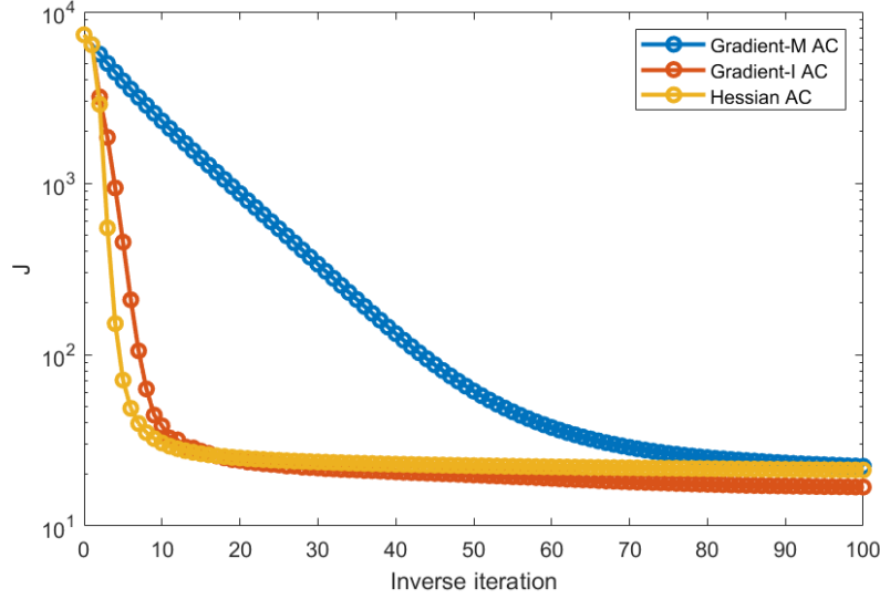
Figure 6.13: An example showing cost function reduction as a function of inverse iterations, when inverting for both A and C using a gradient based approach with l^2 and L^2 gradients, labelled with I and M respectively, and using a Hessian-based inversion where the Hessians of the regularisation terms are exact, and the Hessian of the A and C terms of the misfit are approximated using the fixed-point approach. See section 6.10, for discussion of the l^2 and L^2 gradients.
