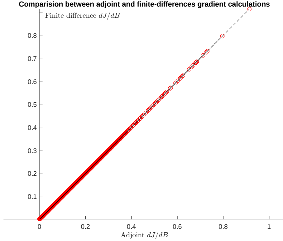
Figure 6.16: Comparison between adjoint and finite differences gradient calculations. This test was done for the Hoffsjökull ice cap in Iceland.
