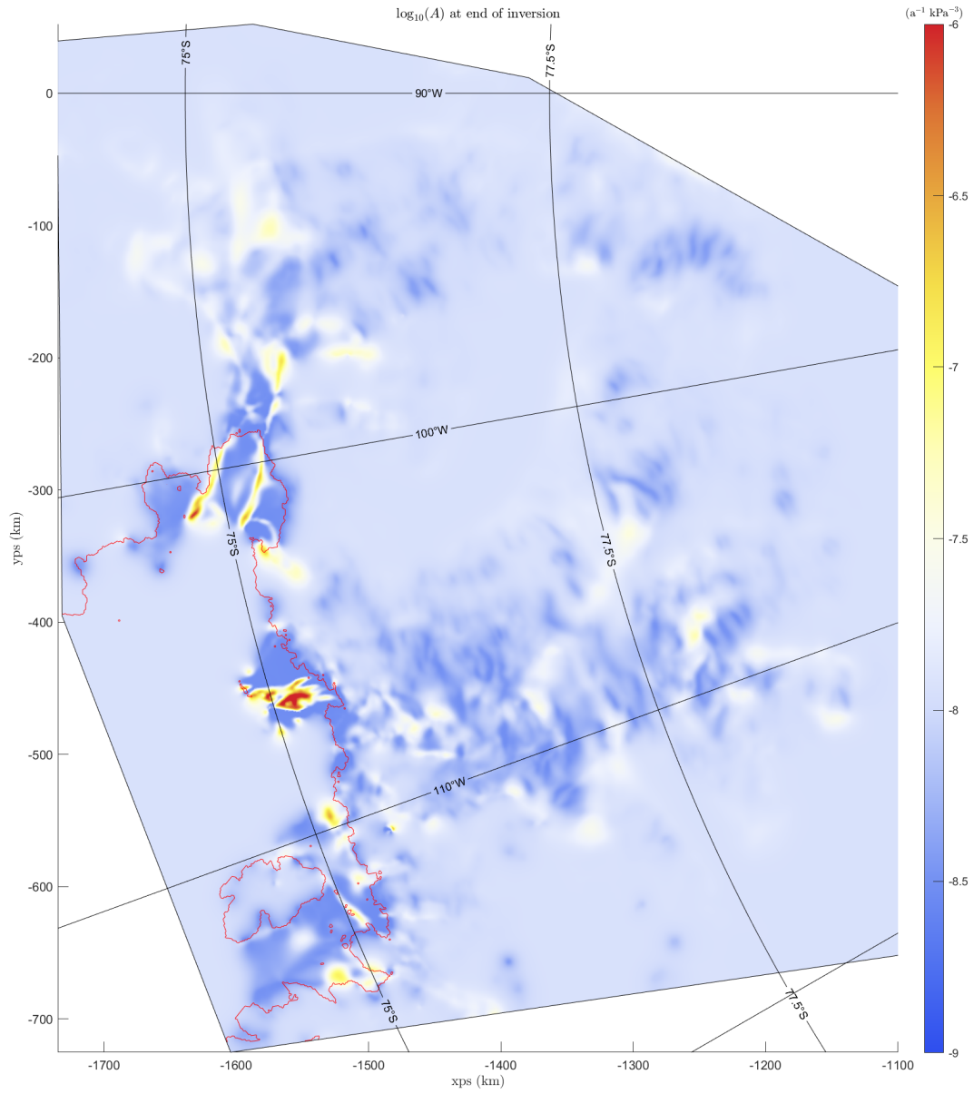
Figure 6.5: Example of an estimated A distribution over section of West Antarctica for n = 3 . Here \gamma_a = 1 and \gamma_s = 100,000 .
