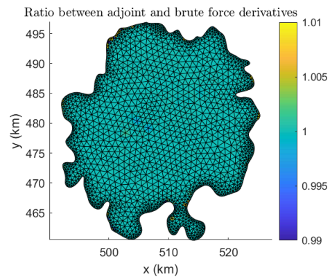
Figure 6.19: Gradient calculation, dJ/dC , done with adjoint and finite differences. This test was done for the Hoffsjökull ice cap in Iceland.
