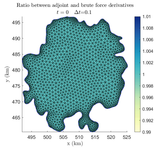
Figure 6.18: Gradient calculation, dJ/dB , done with adjoint and finite differences. This test was done for the Hoffsjökull ice cap in Iceland.
