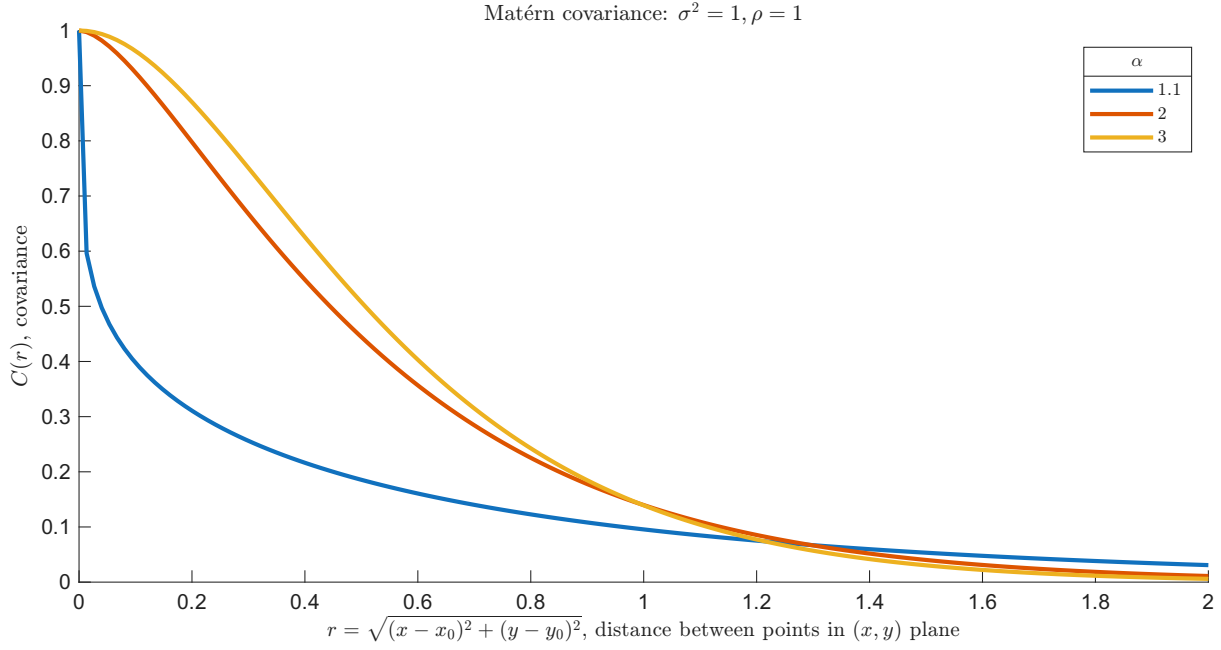
Figure 6.14: The Matérn covariance function, see Eq. (6.52). For \alpha \rightarrow 1 and d = 2 , and \sigma kept held fixed, the field decorrelates at any fixed distance, the correlation length approaches zero.
