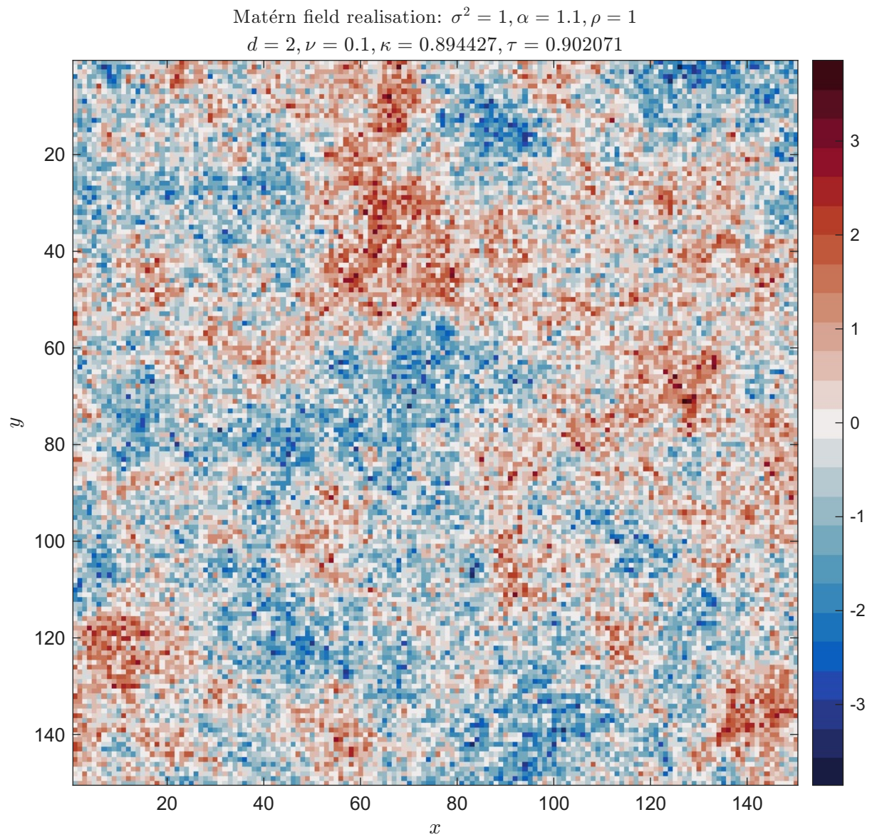
Figure 6.15: An example of a Matérn realisation for \alpha = 1.1 and d = 2 , \sigma = 1 , \rho = 1 . The field is poorly correlated and very rough.
