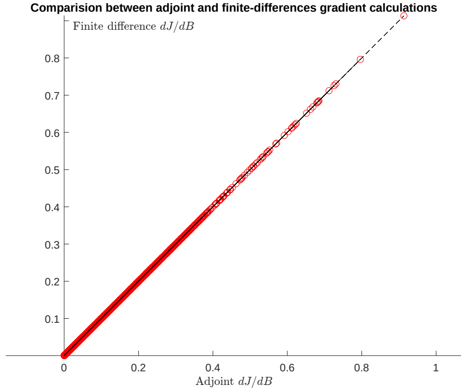
Figure 6.20: Comparison between adjoint and finite differences gradient calculations. This test was done for the Hoffsjökull ice cap in Iceland.
