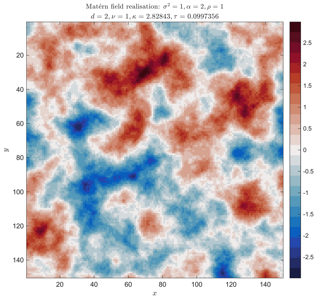
Figure 6.16: An example of a Matérn realisation for \alpha = 2 and d = 2 , \sigma = 1 and \rho = 1 .
