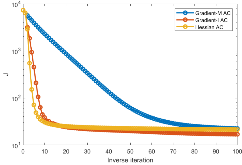
Figure 6.17: An example showing cost function reduction as a function of inverse iterations, when inverting for both A and C using a gradient based approach with l^2 and L^2 gradients, labelled with I and M respectively, and using a Hessian-based inversion where the Hessians of the regularisation terms are exact, and the Hessian of the A and C terms of the misfit are approximated using the fixed-point approach. See section 6.10, for discussion of the l^2 and L^2 gradients.
