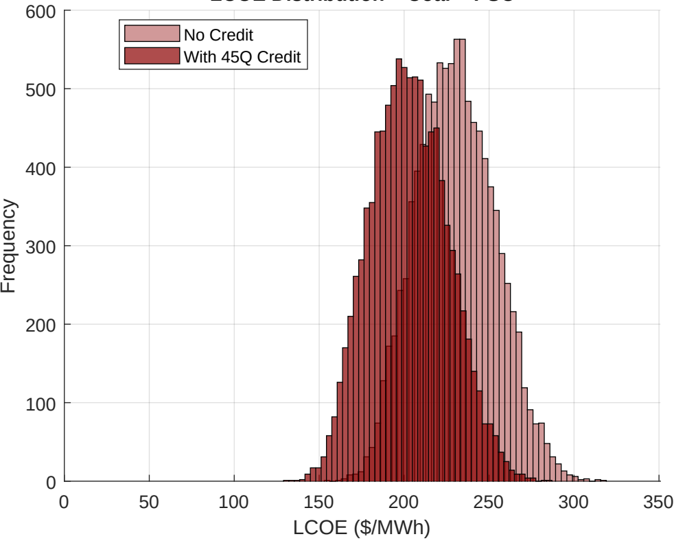
LCOE Distribution – Coal + PSC
