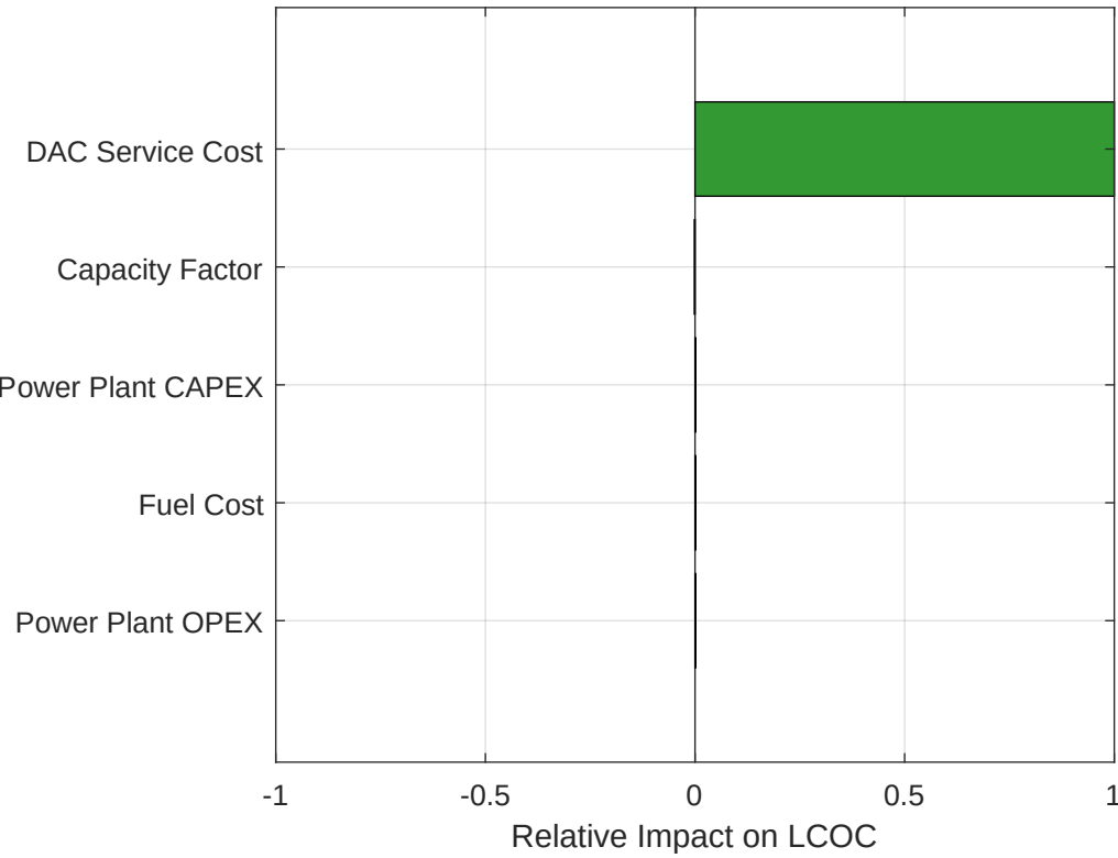
Input Sensitivity on LCOC (With Credit) – NGCC + DAC
