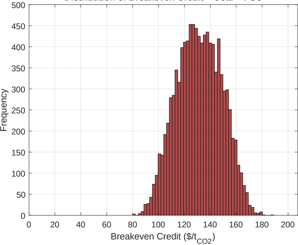
Distribution of Breakeven Credit – Coal + PSC
