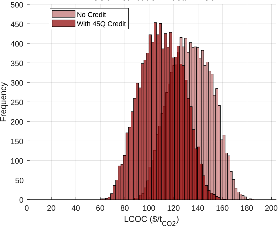
LCOC Distribution – Coal + PSC
