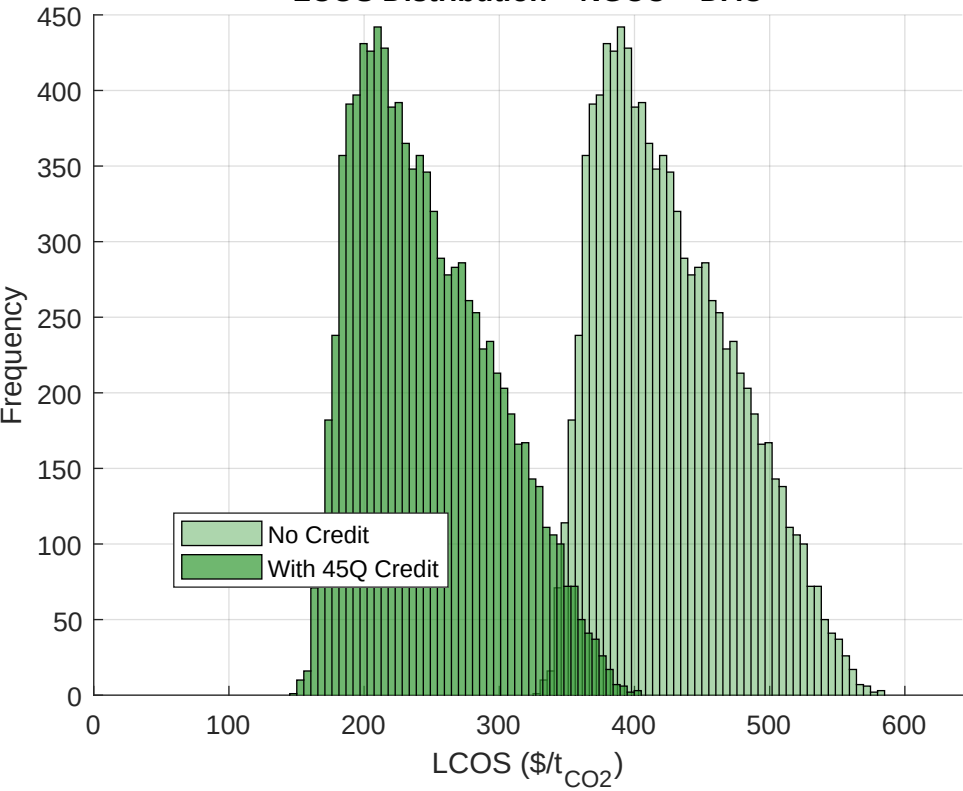
LCOS Distribution - NGCC + DAC
