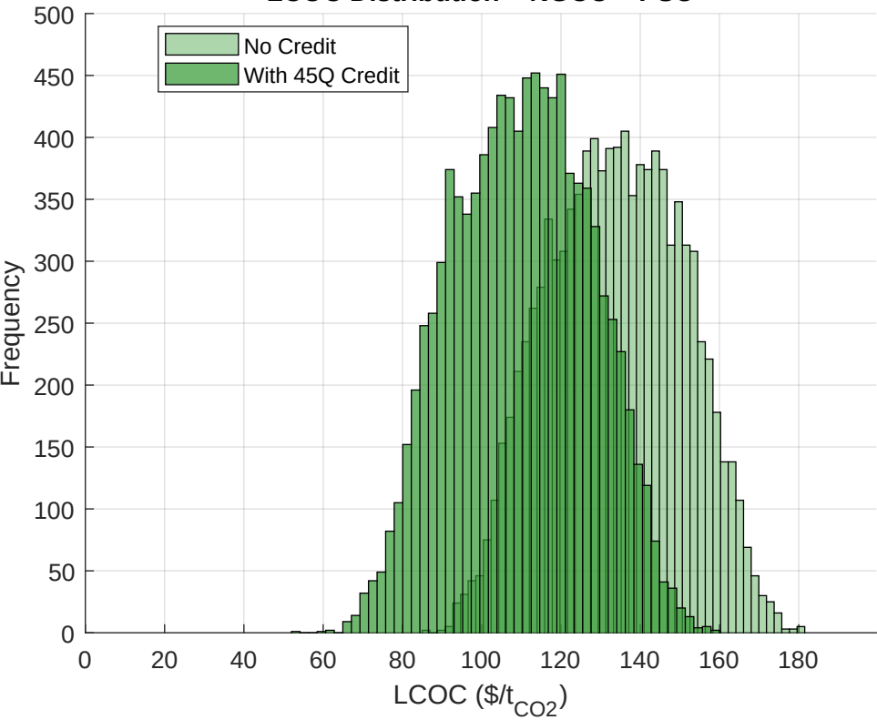
LCOC Distribution – NGCC + PSC
