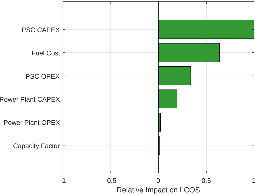
Input Sensitivity on LCOS (With Credit) – NGCC + PSC
