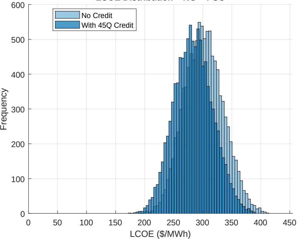
LCOE Distribution – NG + PSC
