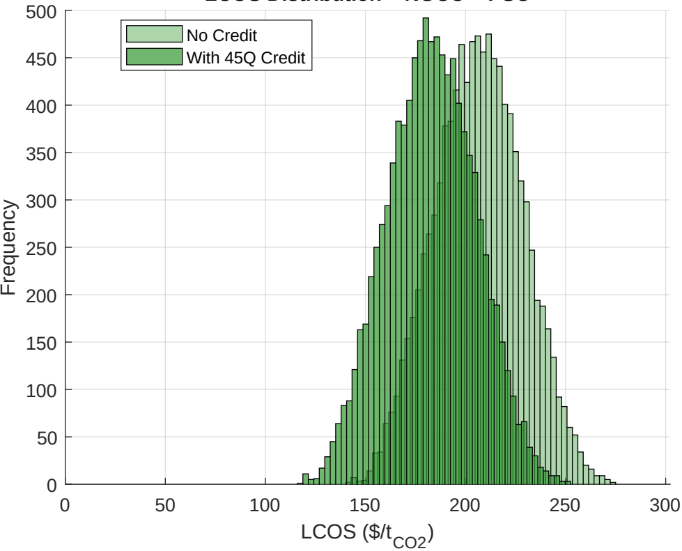
LCOS Distribution - NGCC + PSC
