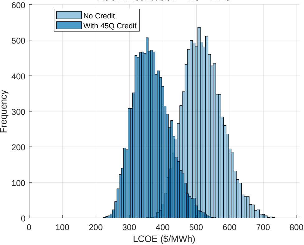
LCOE Distribution – NG + DAC
