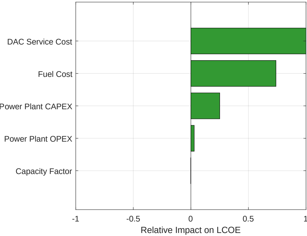
Input Sensitivity on LCOE (With Credit) – NGCC + DAC
