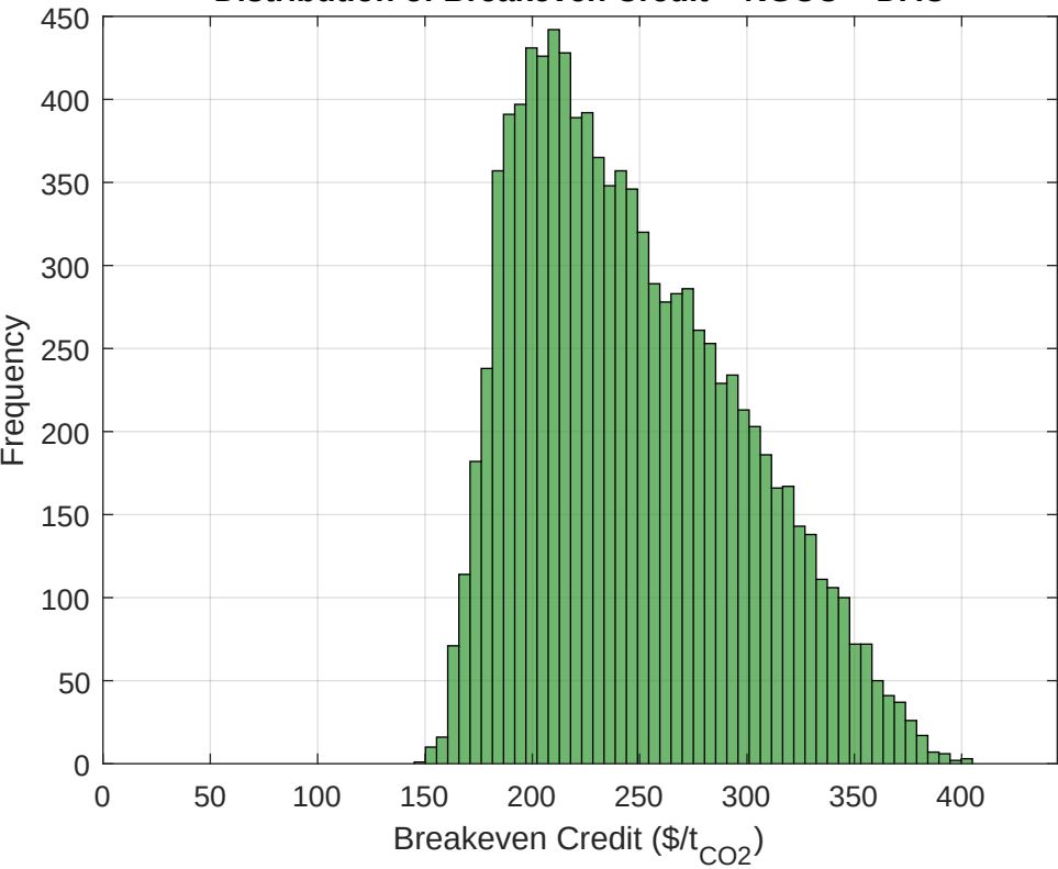
Distribution of Breakeven Credit – NGCC + DAC
