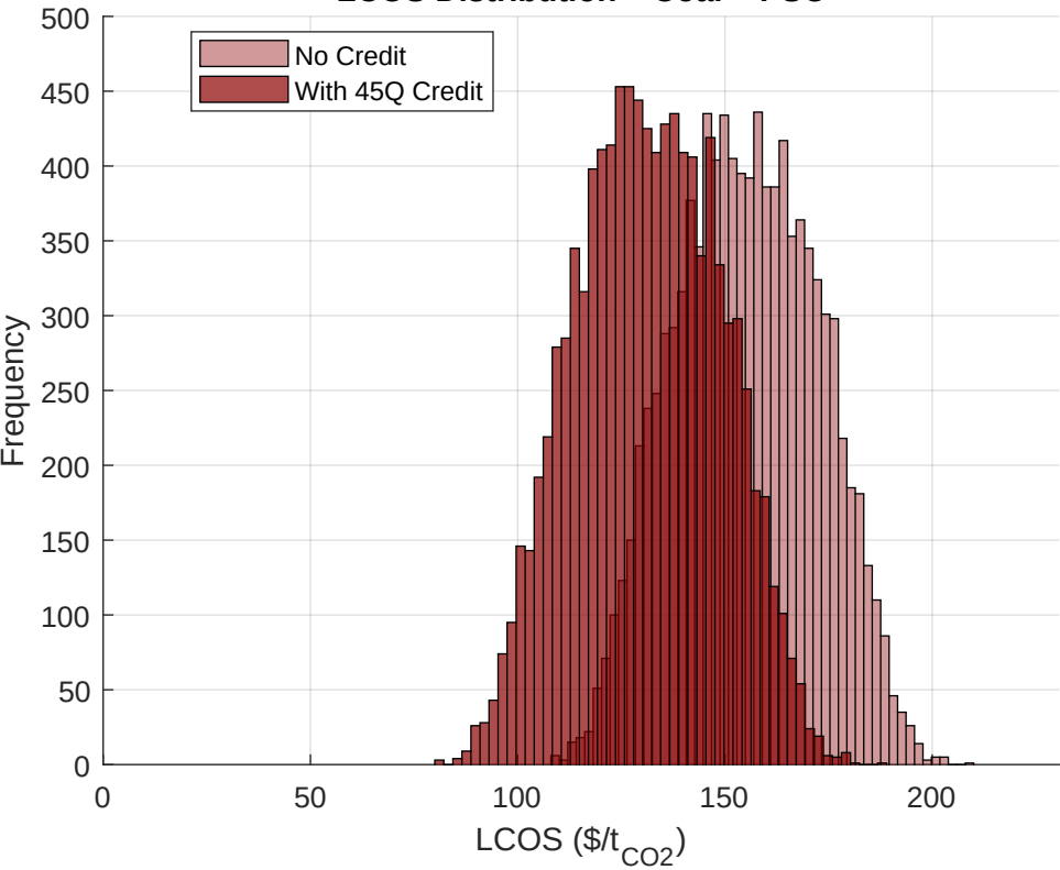
LCOS Distribution – Coal + PSC
