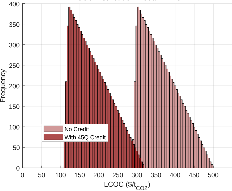
LCOC Distribution – Coal + DAC
