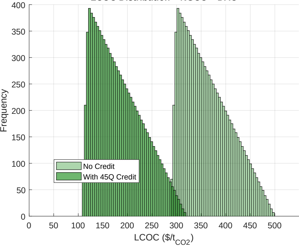
LCOC Distribution – NGCC + DAC
