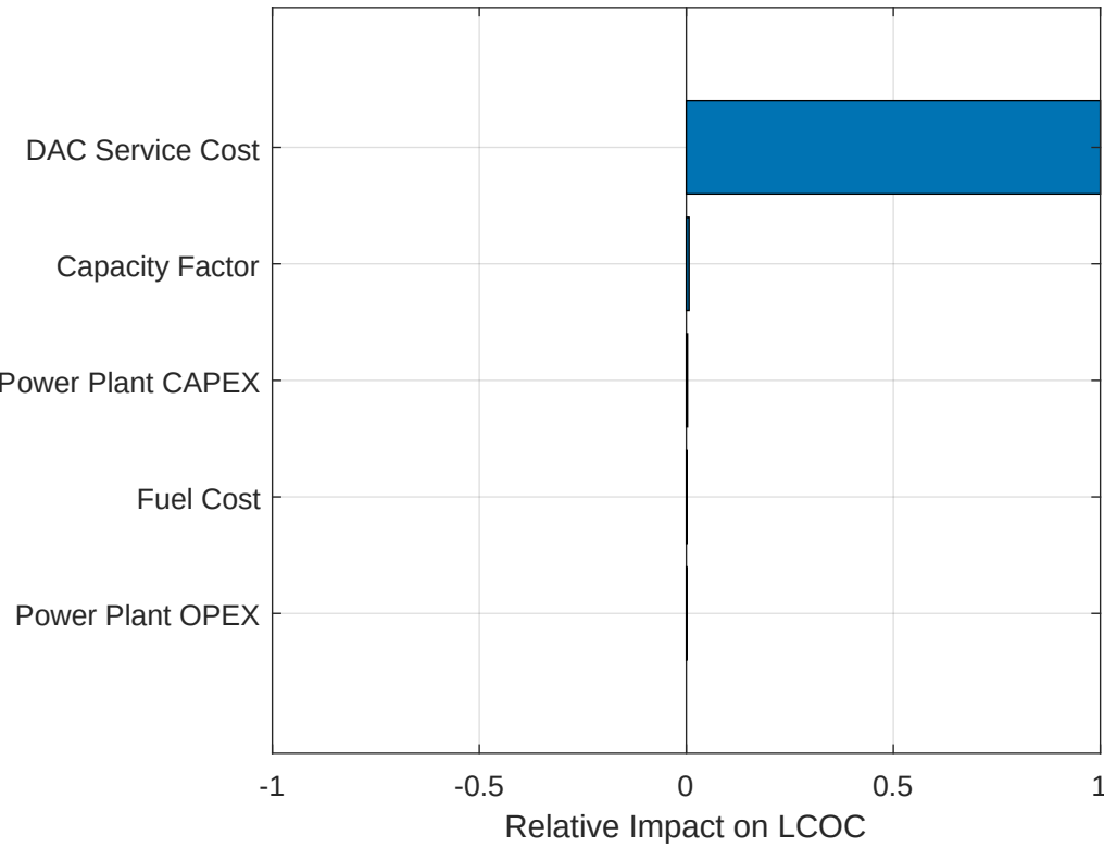
Input Sensitivity on LCOC (With Credit) – NG + DAC
