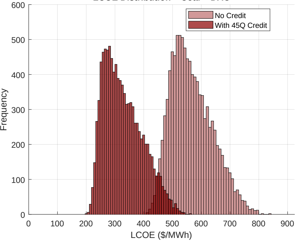
LCOE Distribution - Coal + DAC
