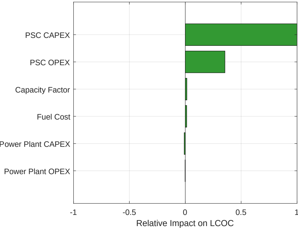
Input Sensitivity on LCOC (With Credit) – NGCC + PSC
