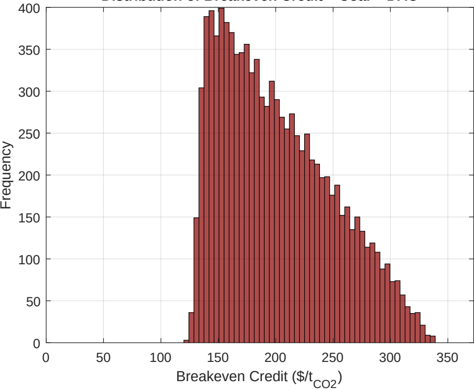
Distribution of Breakeven Credit – Coal + DAC
