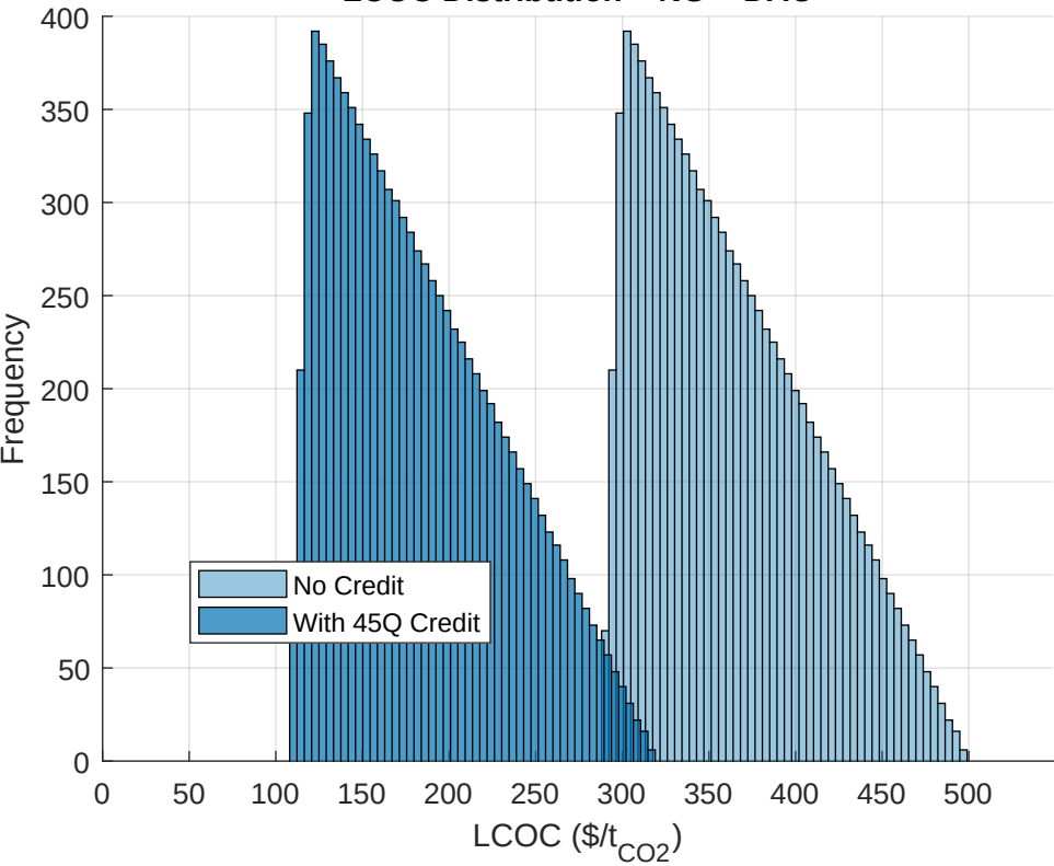
LCOC Distribution – NG + DAC
