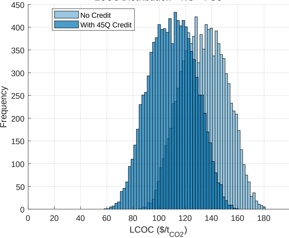
LCOC Distribution – NG + PSC
