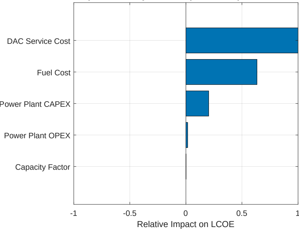
Input Sensitivity on LCOE (With Credit) – NG + DAC
