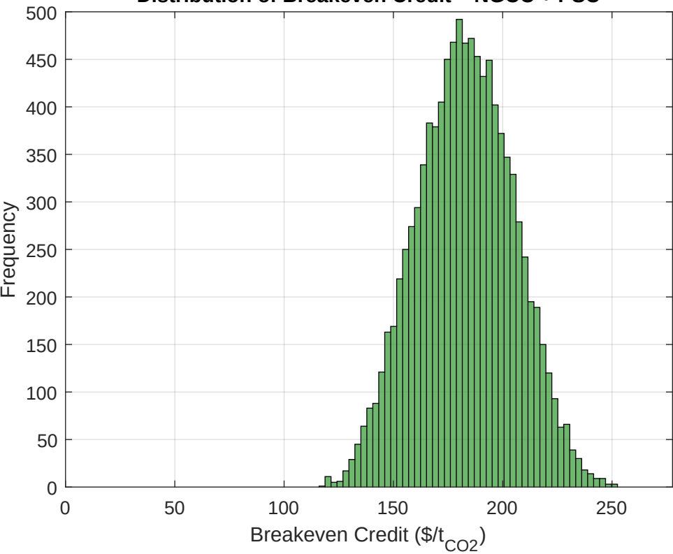
Distribution of Breakeven Credit – NGCC + PSC
