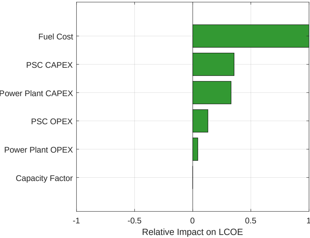
Input Sensitivity on LCOE (With Credit) – NGCC + PSC
