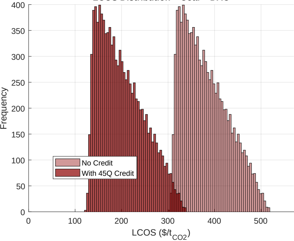
LCOS Distribution – Coal + DAC
