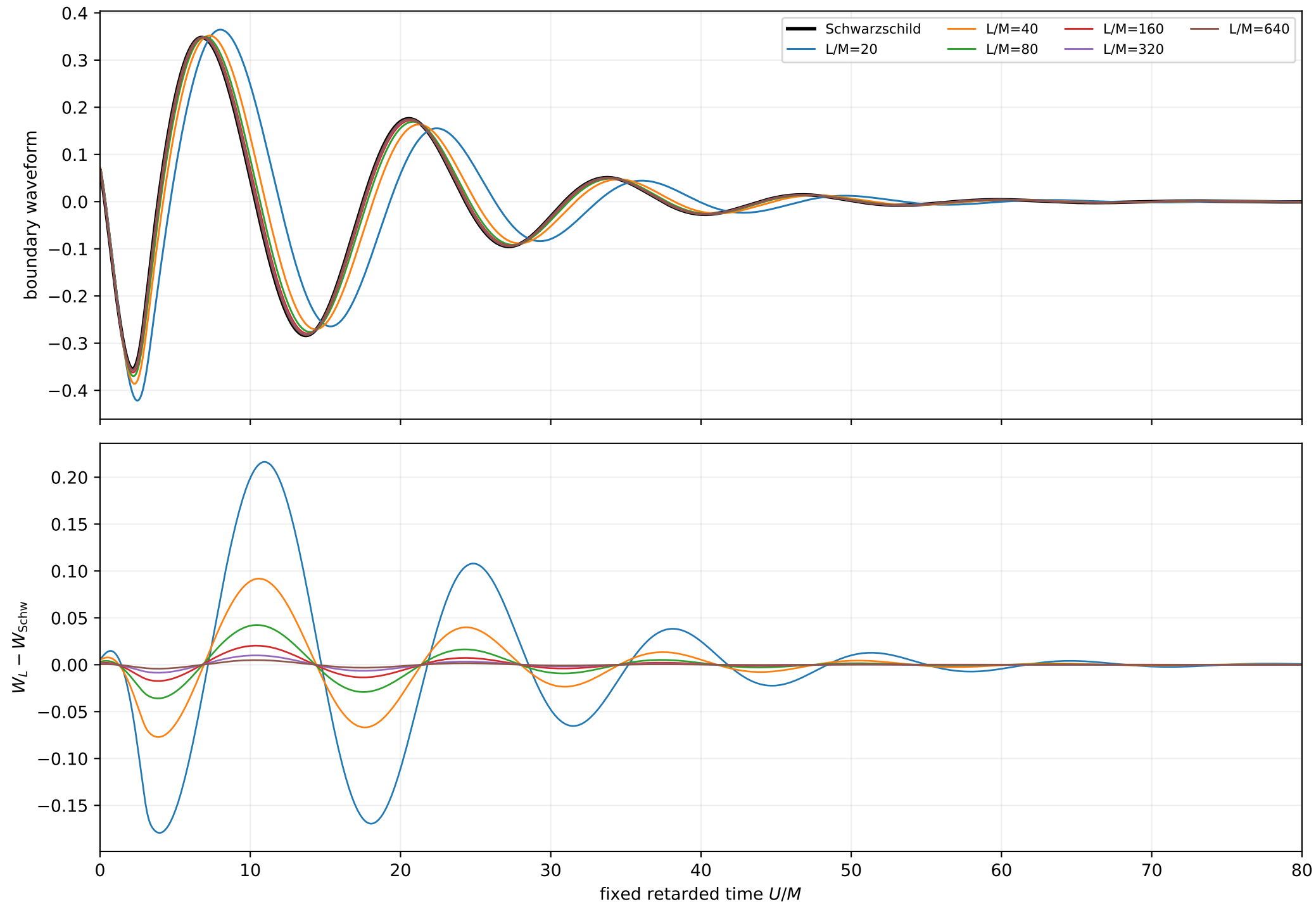
Fixed-data artificial-cosmology waveform sequence
