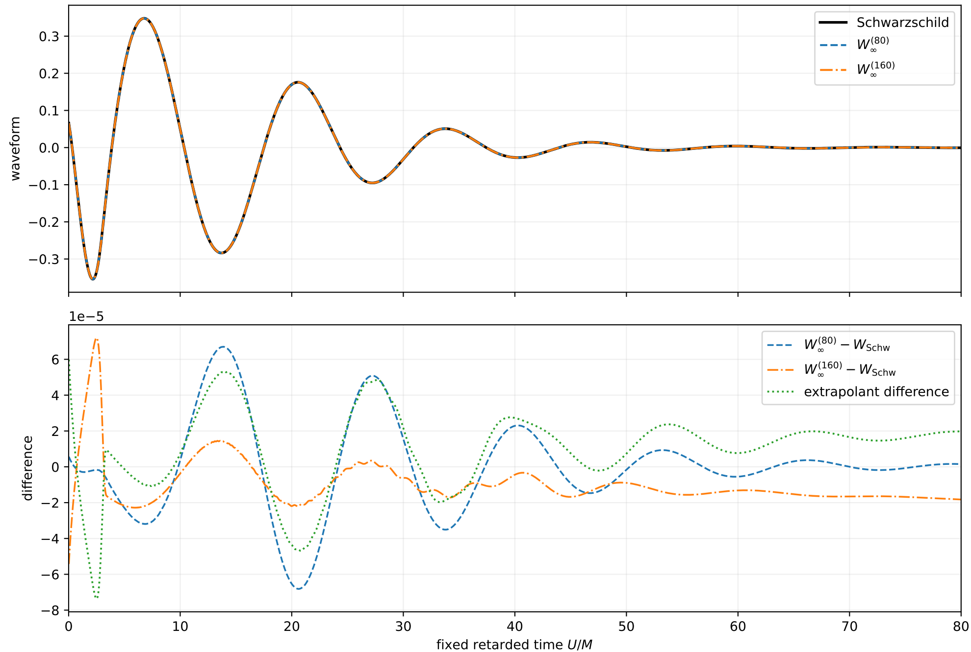
Nested regulator extrapolants and direct Schwarzschild waveform
