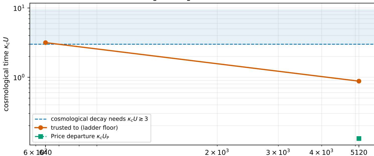
What each cosmological length can reach before its ladder floor
