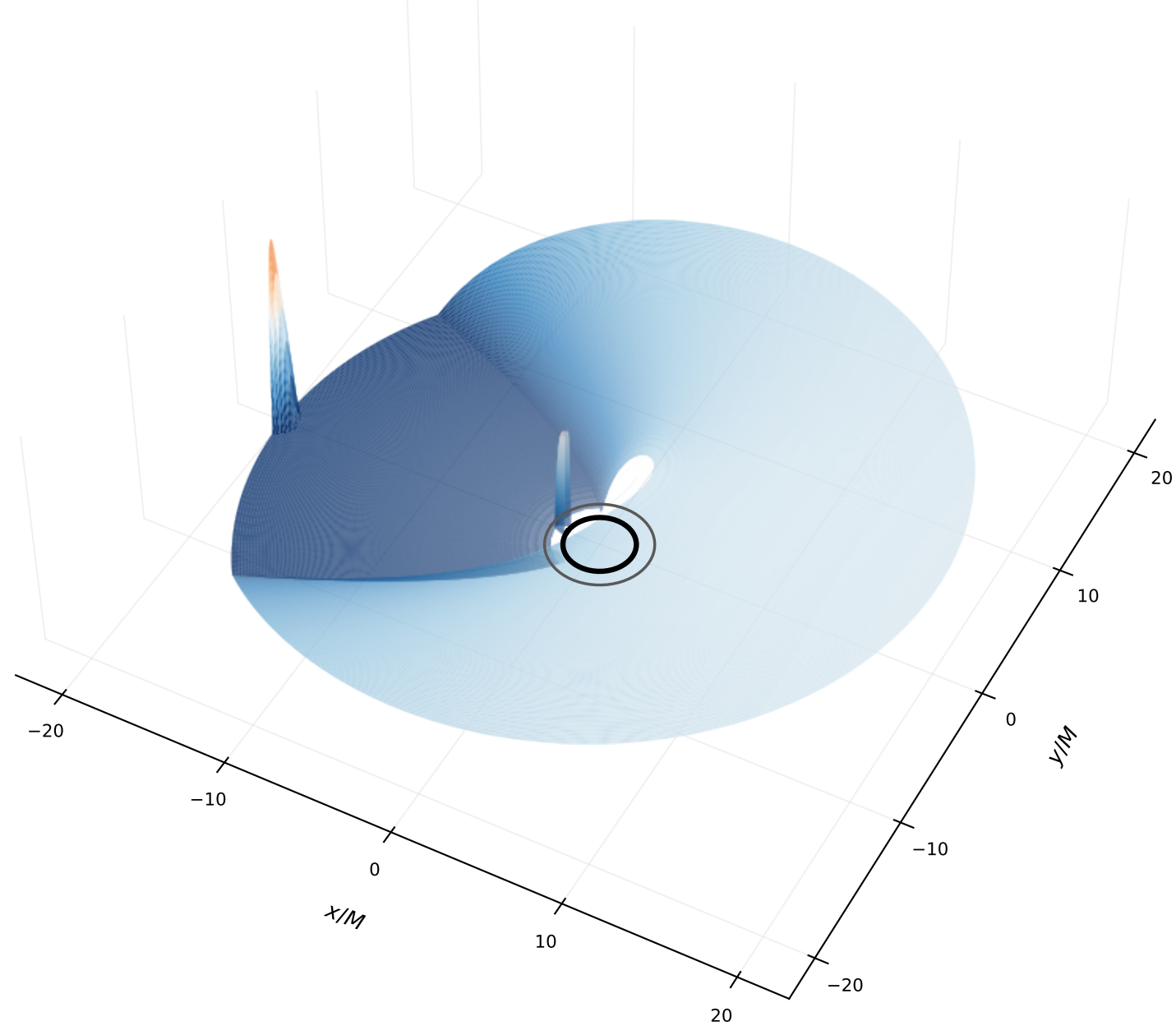
Wavefront as height and colour, \tau/M = 48.00 , clipped at \pm 2.2e - 04
