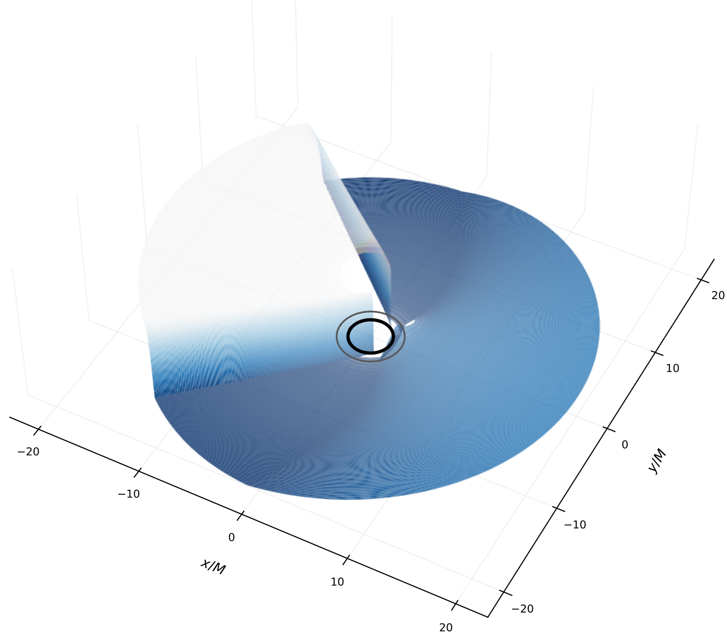
Wavefront as height and colour, \tau/M = 40.00 , clipped at \pm 2.1e - 05
