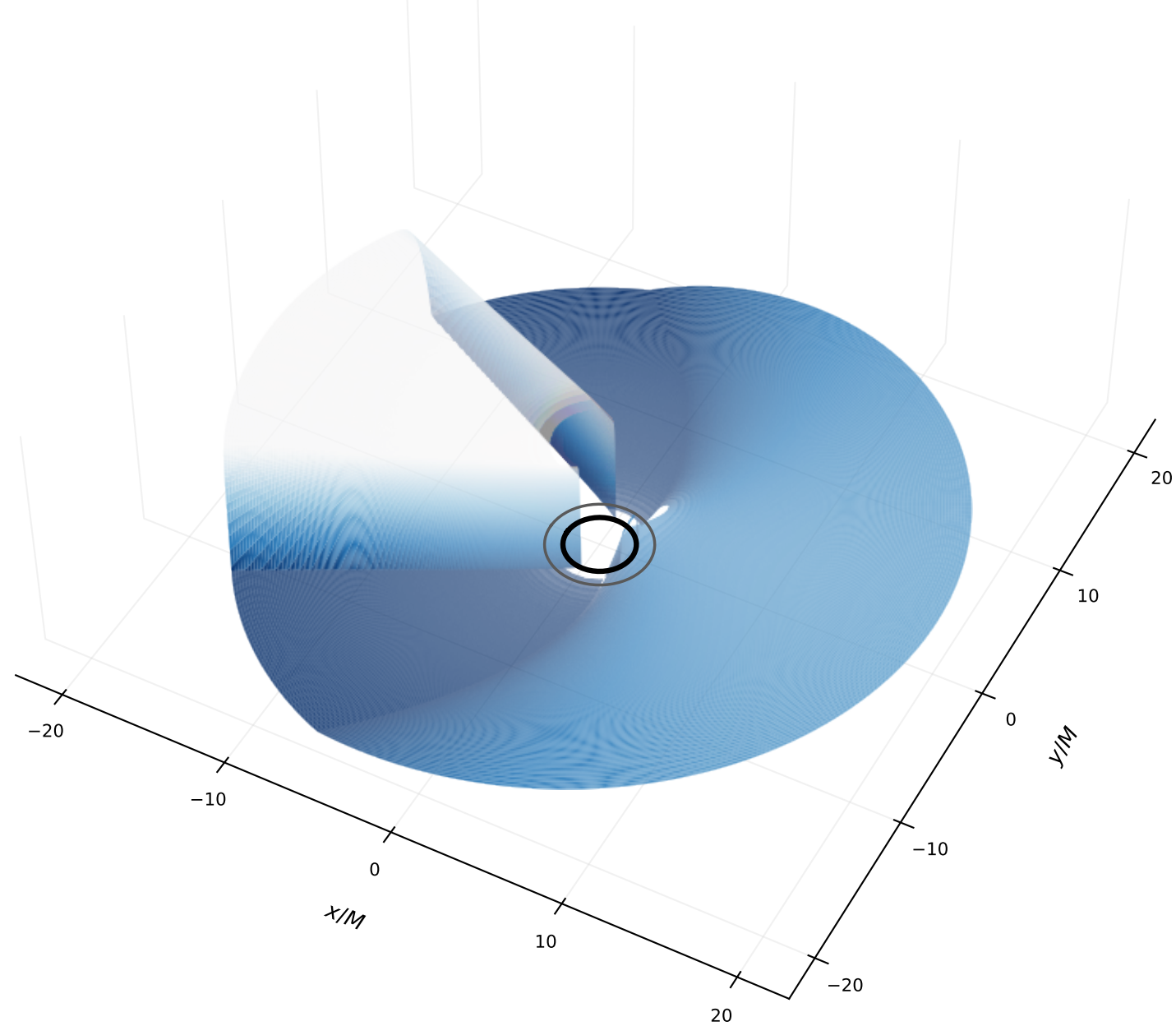
Wavefront as height and colour, \tau/M = 42.00 , clipped at \pm 3.1e - 05
