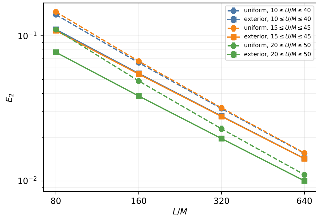
QNM-window disagreement with Schwarzschild
