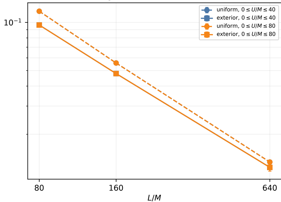
Raw disagreement with Schwarzschild
