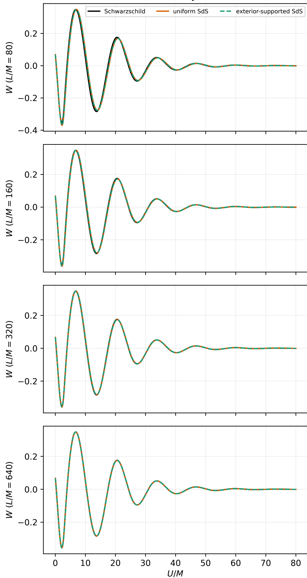
Raw outer-boundary waveforms
