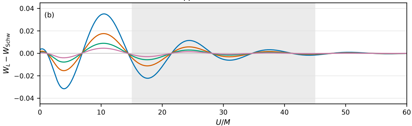
Exterior-supported Schwarzschild-de Sitter
