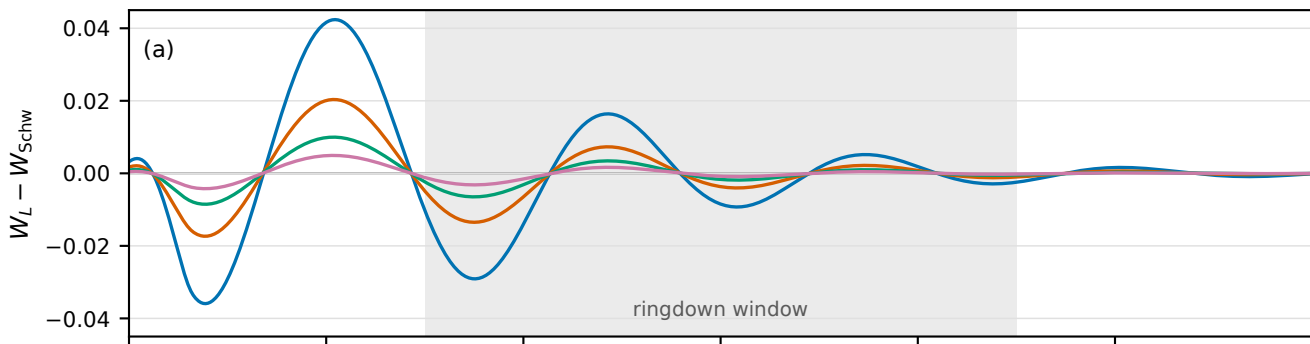
Uniform Schwarzschild-de Sitter
