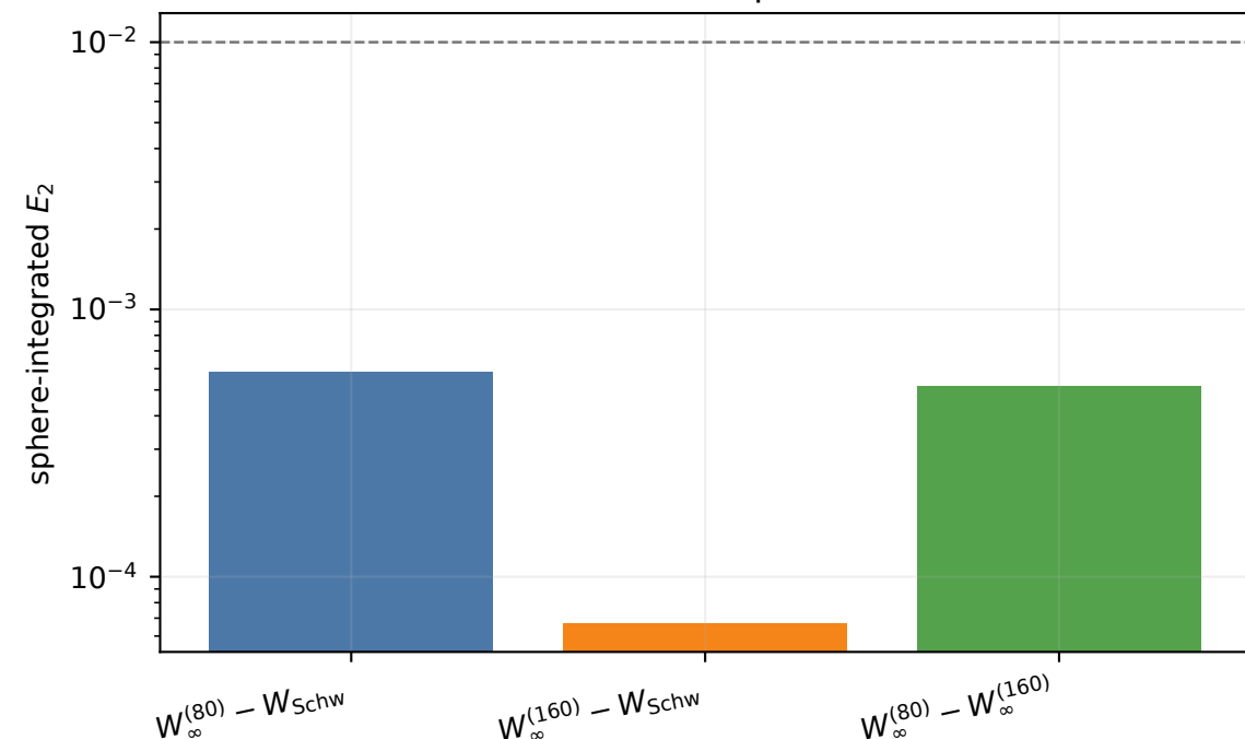
Nested extrapolants
