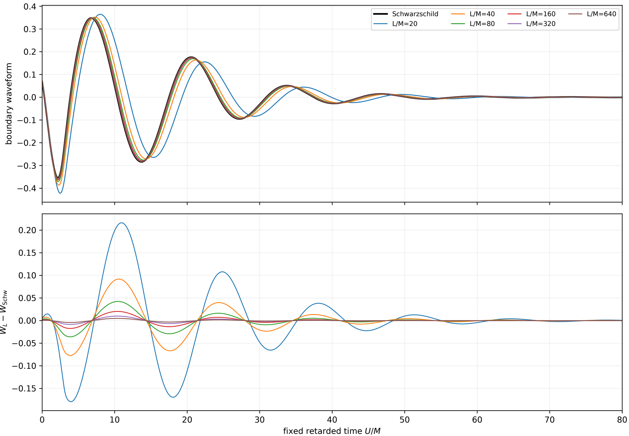
Pure \ell = 2 fixed-data finite- L sequence
