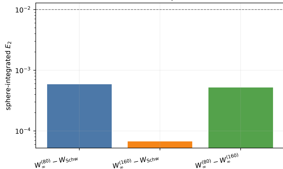
Nested extrapolants
