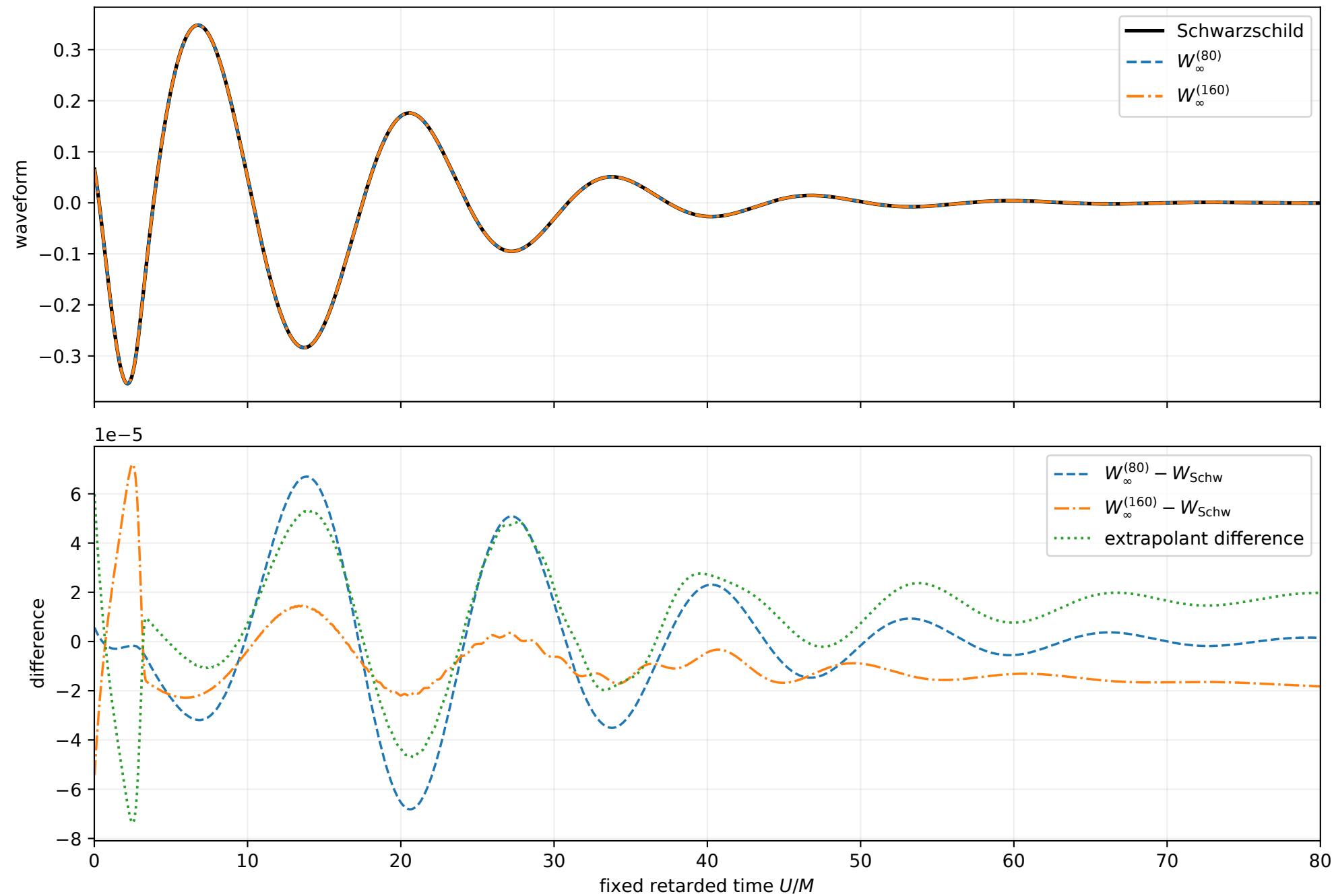
Pure \ell = 2 nested extrapolants and Schwarzschild reference
