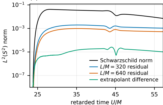
(b) Time-resolved modal norms
