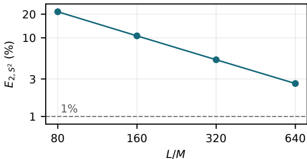
(a) Direct sphere-integrated error
