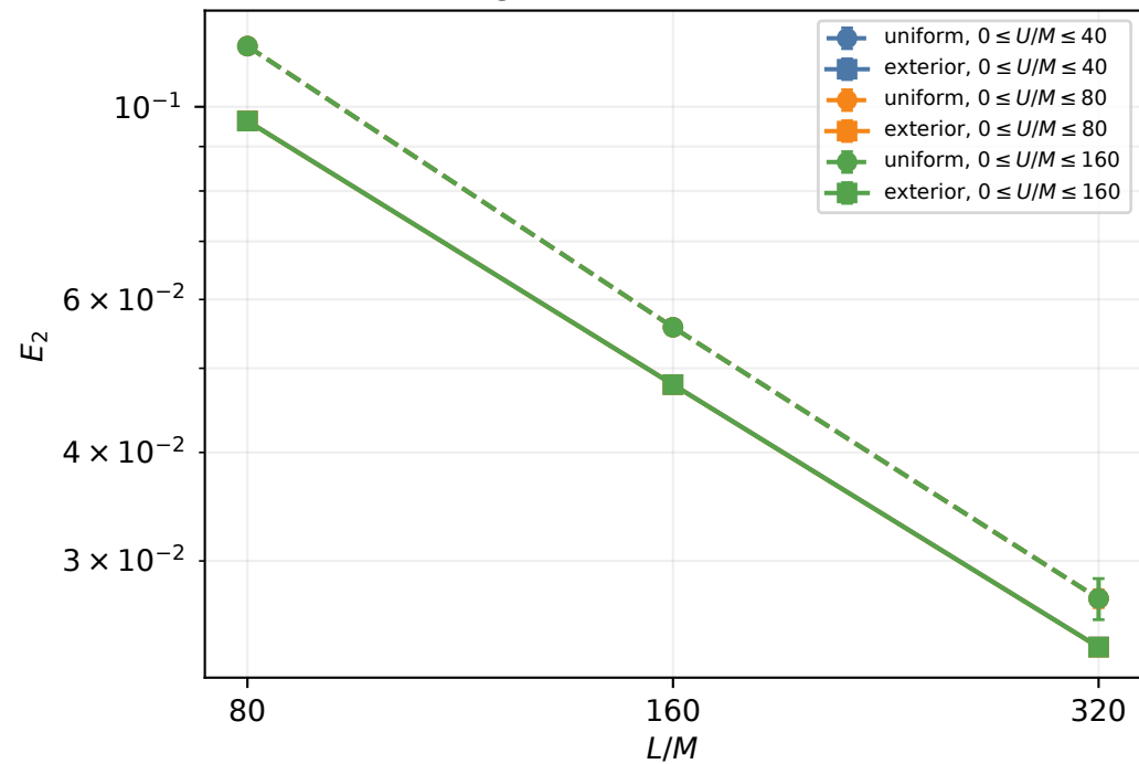
Raw disagreement with Schwarzschild
