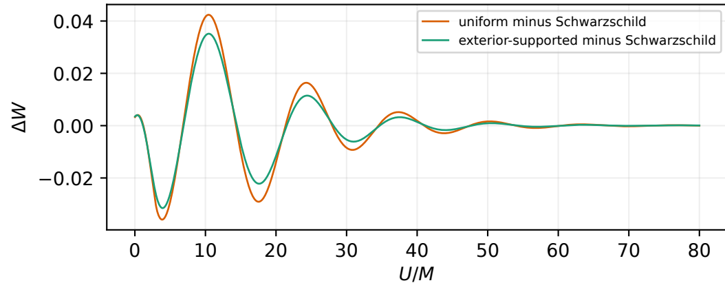
Unshifted residuals from Schwarzschild
