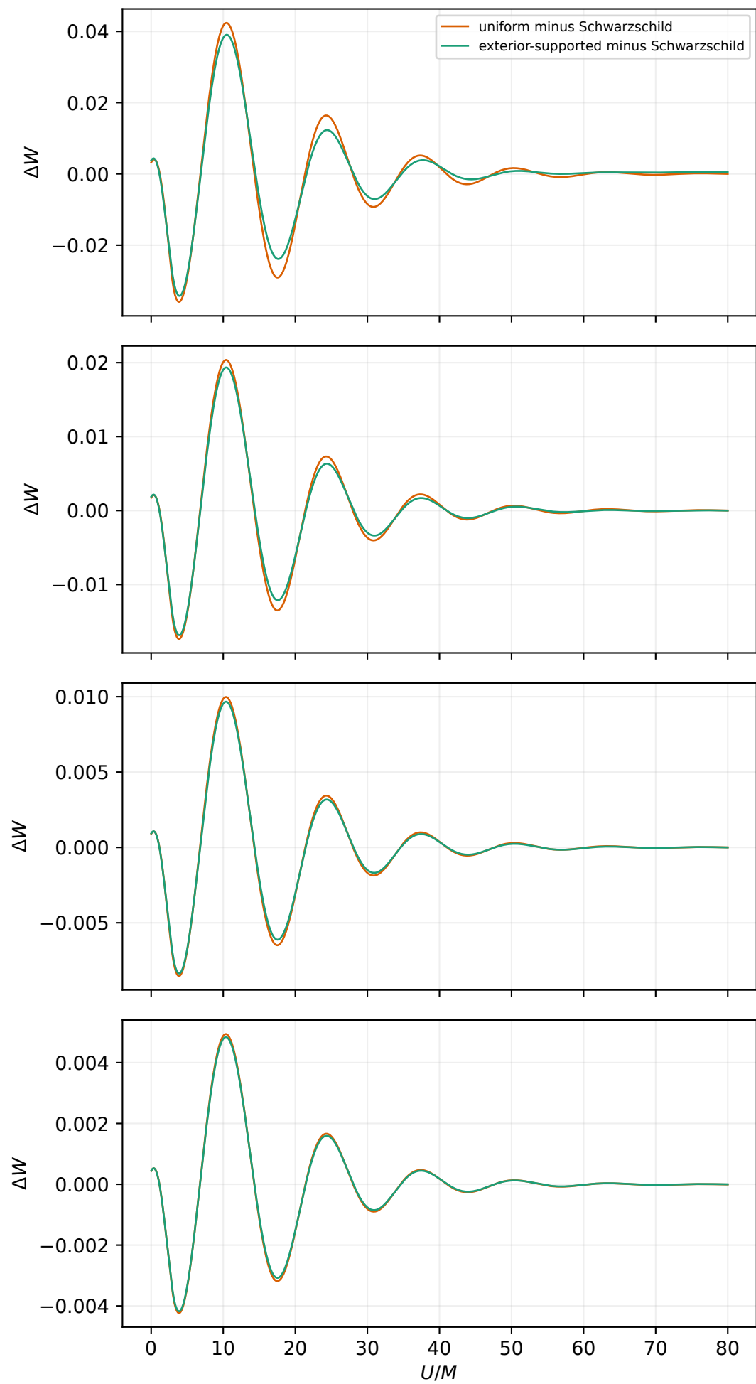
Unshifted residuals from Schwarzschild
